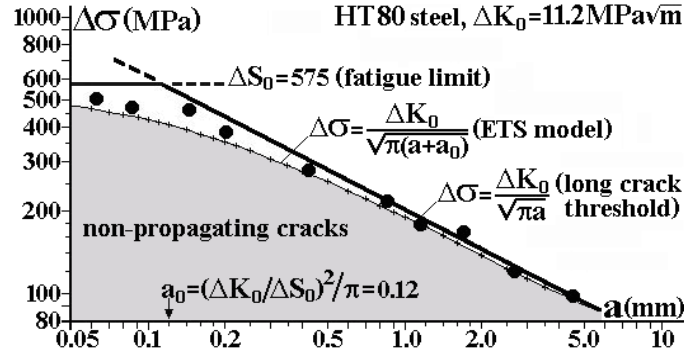
Figure 2: Kitagawa-Takahashi plot describing the fatigue propagation of short and long cracks under pulsating loads ( R = 0 ) in HT80 steel with \Delta K_0 = 11.2 \text{ MPa}\sqrt{\text{m}} and \Delta S_0 = 575 \text{ MPa} .
