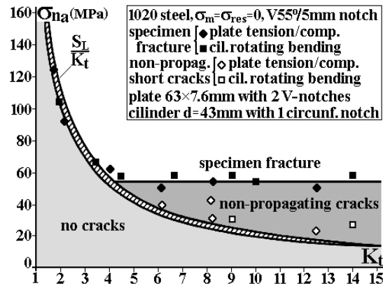
Figure 1: Classical data showing that non-propagating fatigue cracks are generated at the notch roots if S_L/K_t < \sigma_n < S_L/K_f [2, 7].
