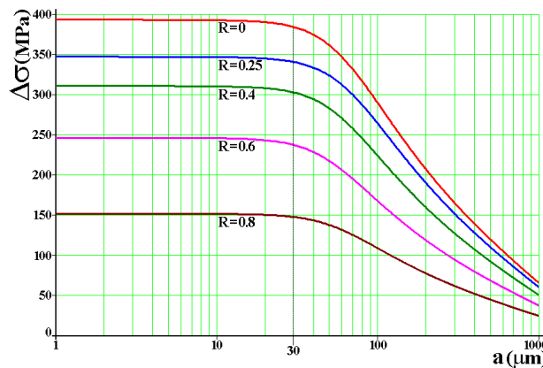
Figure 4: Larger stress ranges tolerable under several R -ratios by the analyzed component considering it contains an edge crack with size a , for w = 3.4mm , \eta = 1.12 , \Delta K_0 = 6MPa\sqrt{m} , a_0 = 59\mu m , \gamma = 6 , and \varphi_F = 1.6 .
