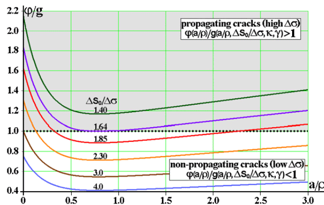
Figure 3: Cracks that can start from the border of a (small) circular hole may propagate by fatigue and then stop if their \varphi/g < 1 .
