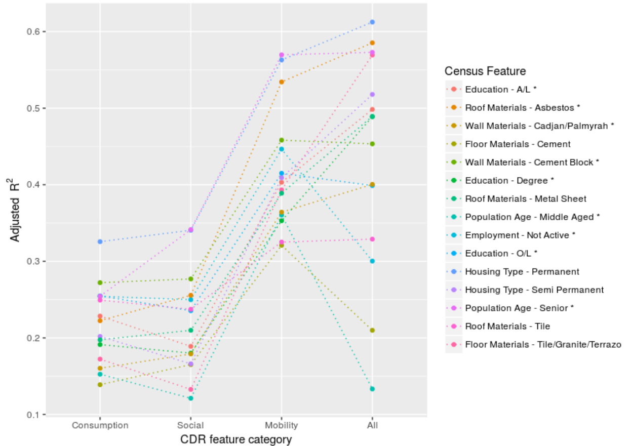
Fig. 2 - Performance of regression models against different variable types
