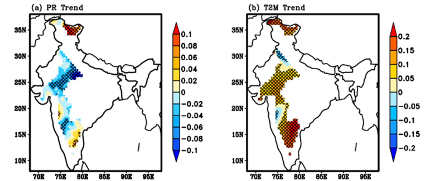
Figure 2: Observed trends in Precipitation and Temperature over semi-arid regions (SARs) of India (1951-2005)
