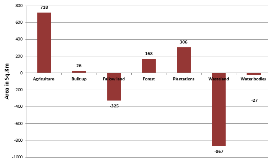
Figure 5: Land-use-Land-cover changes in Mula-Pravara region (1991-2016)
