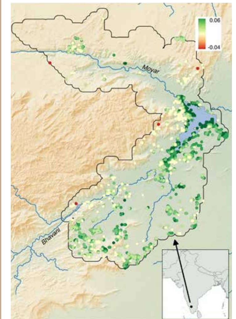
Figure 7: Change in Vegetative Greenness in Moyar-Bhavani Region
