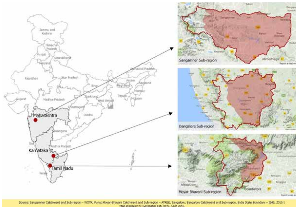
Figure 1: ASSAR Research sites in India
