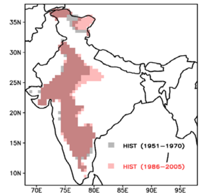
Figure 3: Observed expansion of semi-arid region in India
