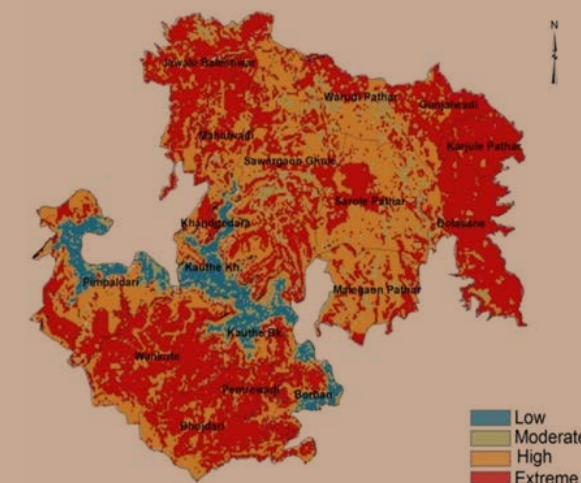
Figure 6: Groundwater Vulnerability classes in 17 villages of Sangamner and Akole, Ahmednagar District.
