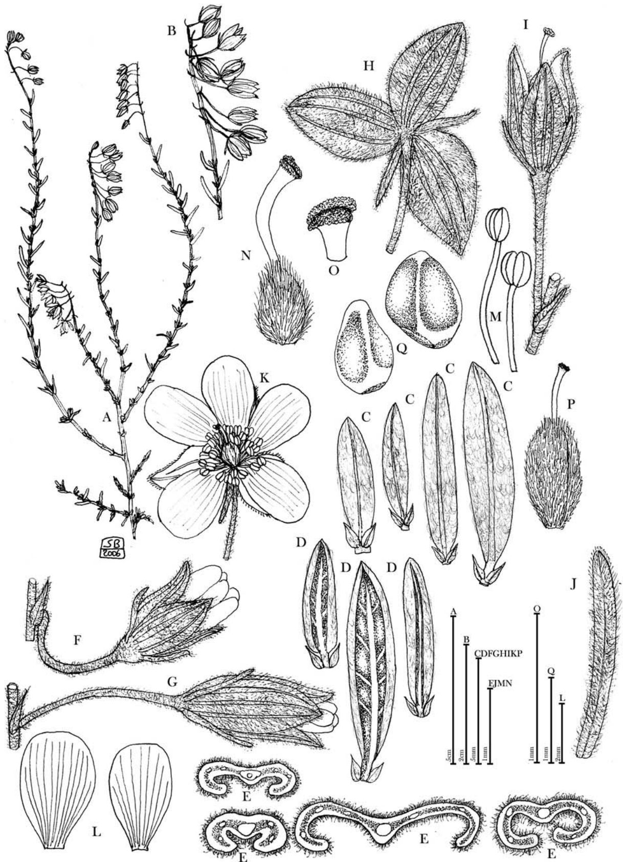
Fig. 1. Helianthemum sicanorum (Holotype, CAT): A , habit; B , detail of inflorescence; C , leaves (upper surface); D , leaves (below surface); E , leaves (transversal section); F , flower bud; G , closed flower; H , open calyx; I , fructified flower; J , terminal part of the outer sepal; K , open flower; L , petals; M , stamens; N , pistil; O , stigma; P , capsule; Q , seeds.
