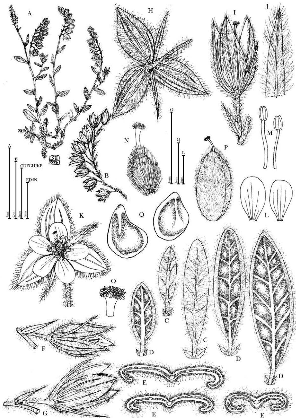
Fig. 4. Helianthemum kahircicum (Libya, CAT): A , habit; B , detail of inflorescence; C , leaves (upper surface); D , leaves (below surface); E , leaves (transversal section); F , flower bud; G , closed flower; H , open calyx; I , fructified flower; J , terminal part of the outer sepal; K , open flower; L , petals; M , stamens; N , pistil; O , stigma; P , capsule; Q , seeds.
