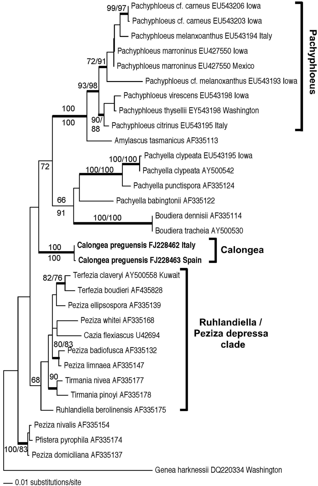
Fig. 1. Most likely tree from maximum likelihood analyses of LSU rDNA with 31 ingroup Pezizaceae. Bootstrap values for significantly supported nodes (>70%) are thickened with parsimony bootstrap on top and likelihood values below. Taxon labels include the Latin binomial followed by the Genbank accession number and geographic origin (when known). Clades of focus in this paper have been labeled.
