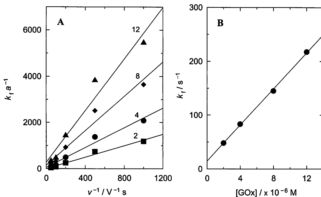
Fig. 3A Plots of the kinetic parameter k_f a^{-1} as a function of v^{-1} for various GOx ox concentrations ( \mu M ) for [Ru(pymq + )(NH 3 ) 5 ] 3+ .
