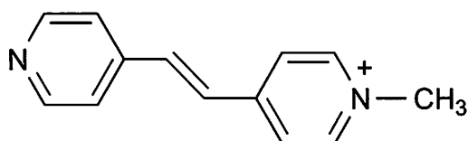
N -methyl-4-[ trans -2-(4-pyridyl)ethenyl]pyridinium ( \text{mebpe}^+ )
