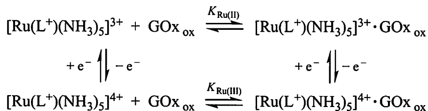
Scheme 1. Adducts formation between [\text{Ru}(\text{L}^+)(\text{NH}_3)_5]^{4+/3+} and GOx ox .
