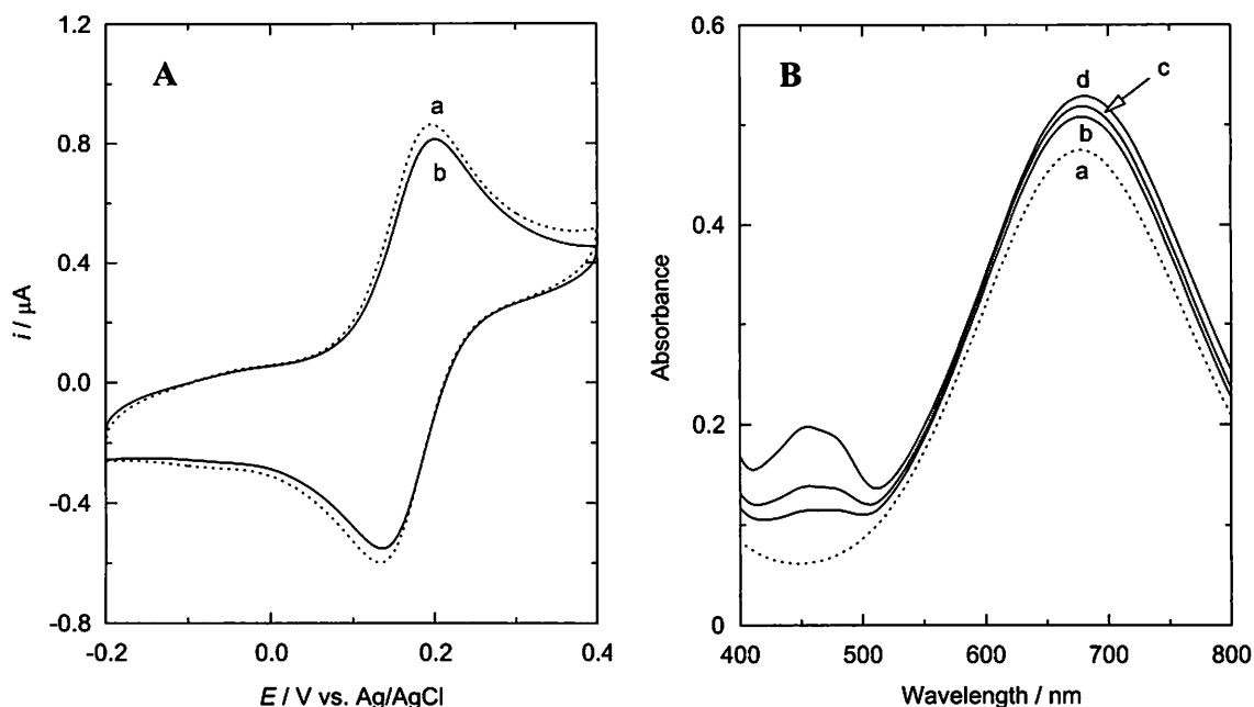
Fig. 4A Cyclic voltammograms of 0.2 mM [Ru(pymq + )(NH 3 ) 5 ] 3+ in 0.1 M phosphate buffer (pH 7.0) in the absence (a) and presence (b) of 0.1 mM GOx ox . Scan rate, 50 mV s -1 .
