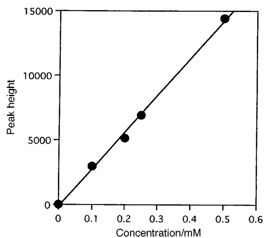
Fig. 5 Calibration graph for pyrene in the range 0.1–0.5 mM.
