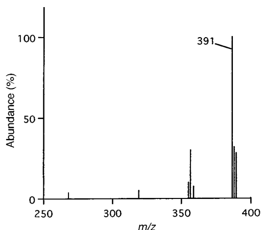
Fig. 2 ESI-MS spectrum of the [coronene-TR + ] ion at drift voltage of 20 V.
