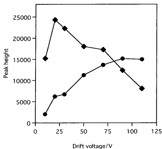
Fig. 1 Variation in peak height of M-TR + and M + ions vs. the drift voltage (V) for pyrene.
