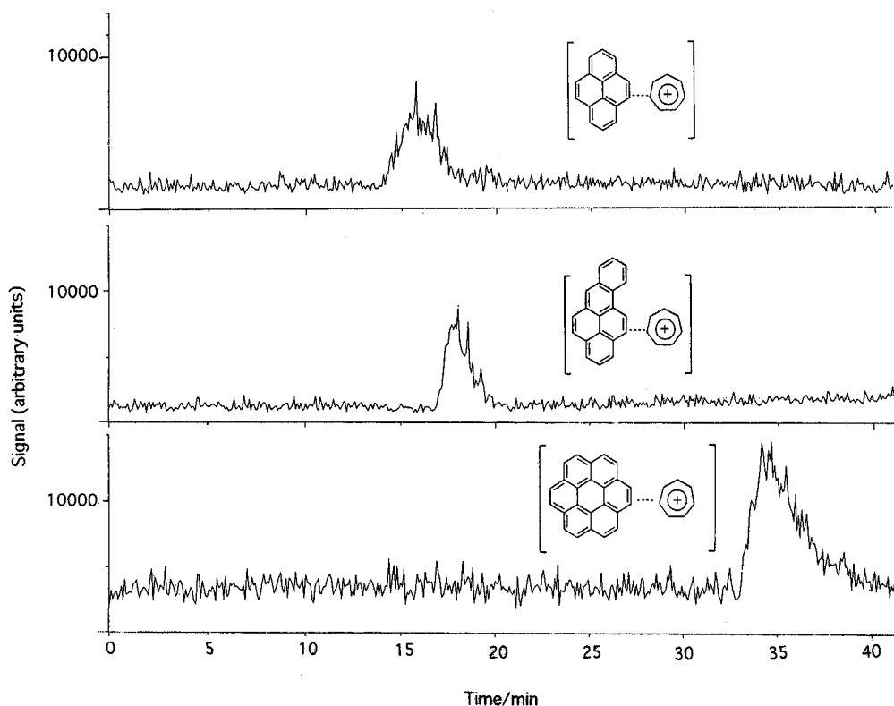
Fig. 4 LC-ESI-MS chromatograms of pyrene, benzo(a)pyrene and coronene for the injection (5 \mu l) of a standard solution of PAHs (0.2, 0.05 and 0.25 mM) by selected-ion monitoring ( m/z 293, 343 and 391, respectively).
