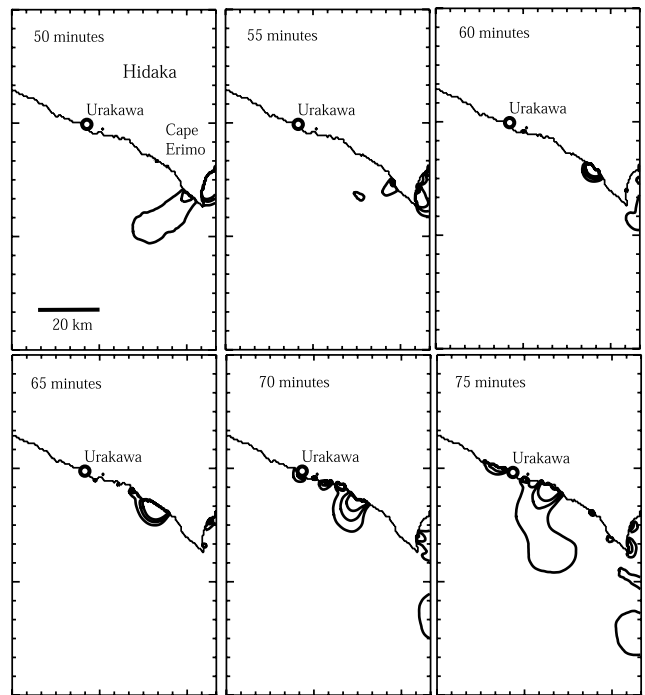
Fig. 5. Six snapshots of the computed tsunami propagation near the west coast of Hidaka area at 50, 55, 60, 65, 70, 75 minutes after the origin time of the earthquake. The contours show the tsunami heights of 15 cm, 30 cm, 45 cm.
