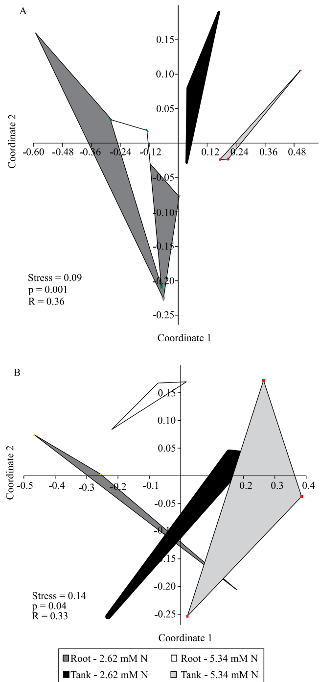
Figure 1. Diagram of non-metric multidimensional scaling (nMDS), considering the ordering of the groups formed by the fertilized organ (roots or tank) and by the concentration of nitrogen applied to the bromeliad species Guzmania lingulata (A) and Vriesea 'Harmony' (B). The stress value is the distortion between the actual data and that plotted in the diagram. The statistical inference of the dissimilarity among groups was obtained with the multivariate technique of one-way analysis of similarity, at 5% probability and with R < 1 .
