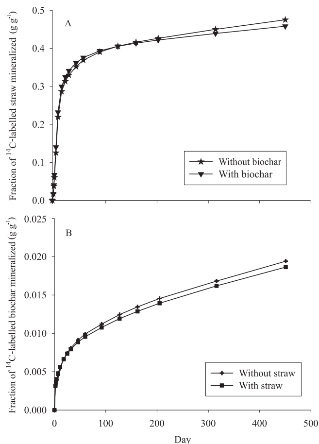
Figure 1. Mineralization: A, labelled straw, with or without addition of biochar; and B, labelled biochar, with or without addition of straw.
