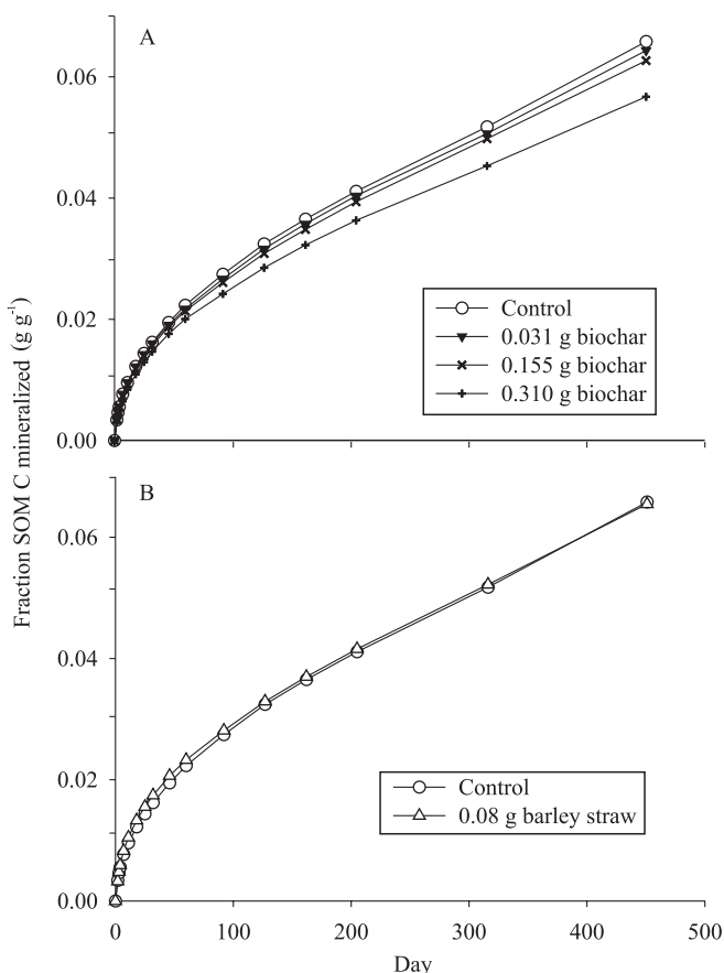
Figure 2. Mineralization of 40-year-old labelled soil organic matter (SOM) with: A, different additions of biochar; and B, with addition of straw.
