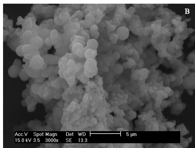
Figure 1. Scanning electron microscope (SEM) micrograph of cellulose raw material (A); and microwave-assisted hydrothermally carbonized cellulose (B).
