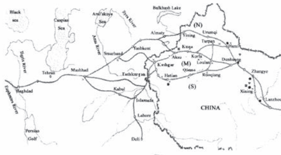
Fig. 2.3. Northwestern Silk Road and ancient Chinese glass distribution. ● PbO-BaO-SiO 2 glass × Na 2 O-CaO-SiO 2 glass ▼ Alkali fayence ■ K 2 O-SiO 2 glass.
