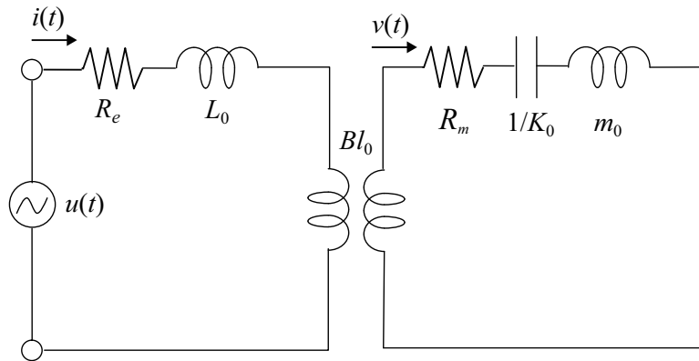
Figure 4-1 Equivalent circuit of loudspeaker system.
