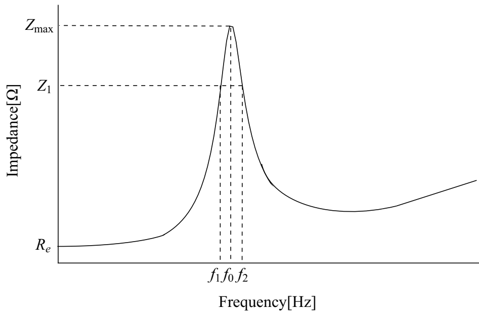
Figure 2-3 Impedance–frequency characteristic.
