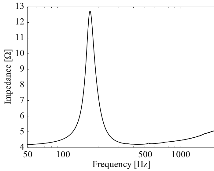
Figure 4-3 Impedance characteristic of a target loudspeaker system.
