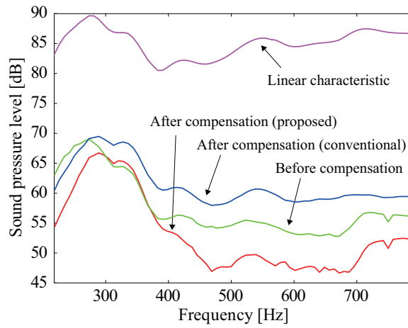
(a) 2nd-order intermodulation distortion (sum)
