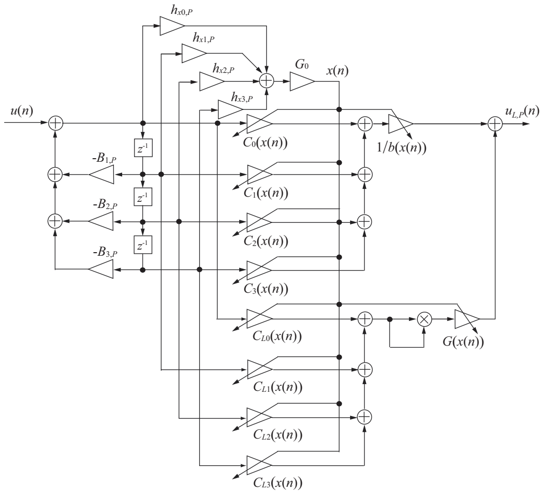
Figure 4-2 Block diagram of 3rd-order nonlinear IIR filter.
