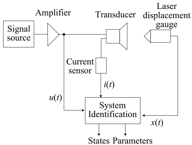
Figure 4-4 Block diagram of Klippel measurement instrument.
