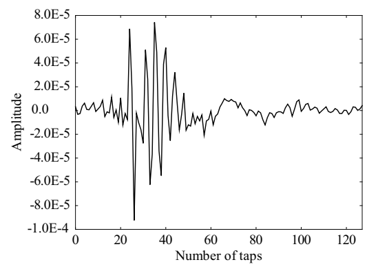
(c) Second-order (main diagonal component)
