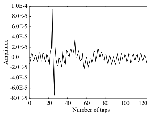
(c) Second-order (main diagonal component)
