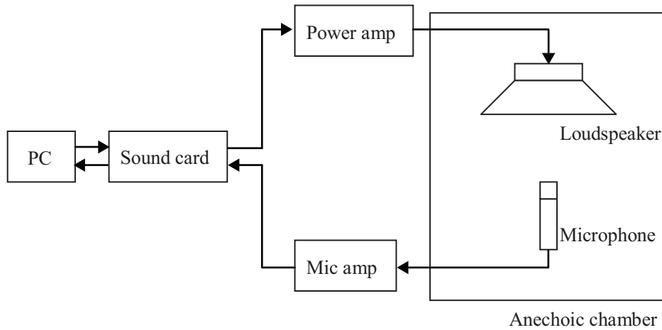
Figure 3-13 Composition of experimental equipment.
