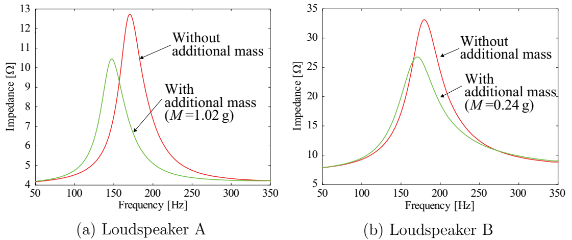
Figure 3-4 Impedance characteristics.
