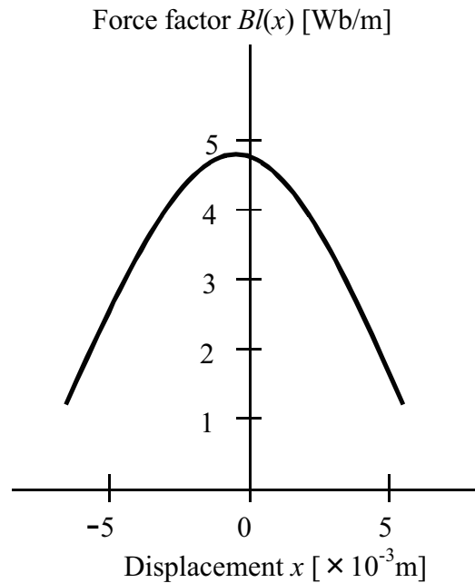
Figure 1-5 Typical force factor BI(x) versus displacement x curve.
