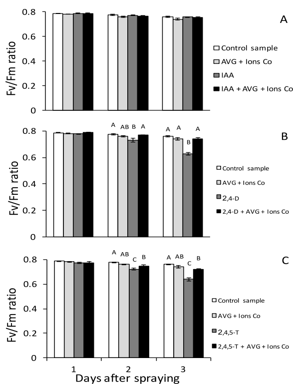
Figure 3 F_v/F_m ratio followed for three days in bean plants treated with: water (Control sample); AVG + Co^{2+} ; IAA; IAA + AVG + Co^{2+} (A); water; AVG + Co^{2+} ; 2,4-D; 2,4-D + AVG + Co^{2+} (B); water; AVG + Co^{2+} ; 2,4,5-T; 2,4,5-T + AVG + Co^{2+} (C).
