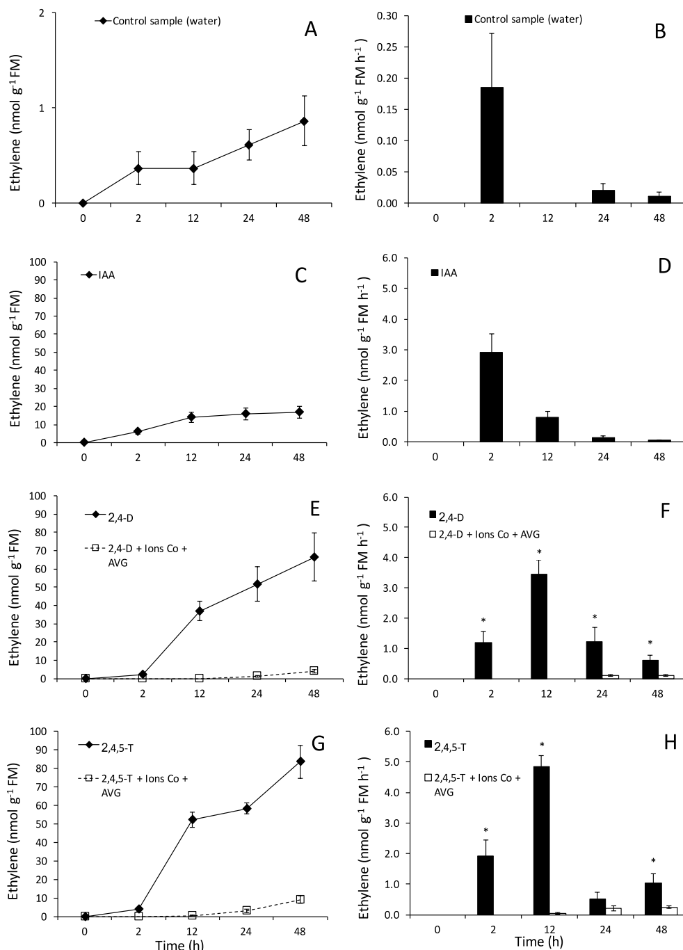
Figure 1 Accumulation (left) and production rate (right) of ethylene in bean plants, two weeks after emergence, treated with: water (Control sample, A and B); IAA; IAA + AVG + Co 2+ (C and D); 2,4-D; 2,4-D + AVG + Co 2+ (E and F); 2,4,5-T; 2,4,5-T + AVG + Co 2+ (G and H). Control sample bean plants plus AVG and Co 2+ and the ones treated with IAA plus AVG and Co 2+ did not produce detectable ethylene.
