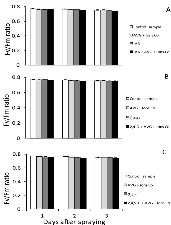
Figure 4 F_v/F_m ratio followed for three days in maize plants treated with: water (Control sample); AVG + Co^{2+} ; IAA; IAA + AVG + Co^{2+} (A); water; AVG + Co^{2+} ; 2,4-D; 2,4-D + AVG + Co^{2+} (B); water; AVG + Co^{2+} ; 2,4,5-T; 2,4,5-T + AVG + Co^{2+} (C).
