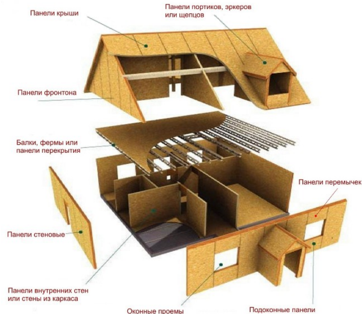
Fig 2. Wooden frame-shield system [2]
