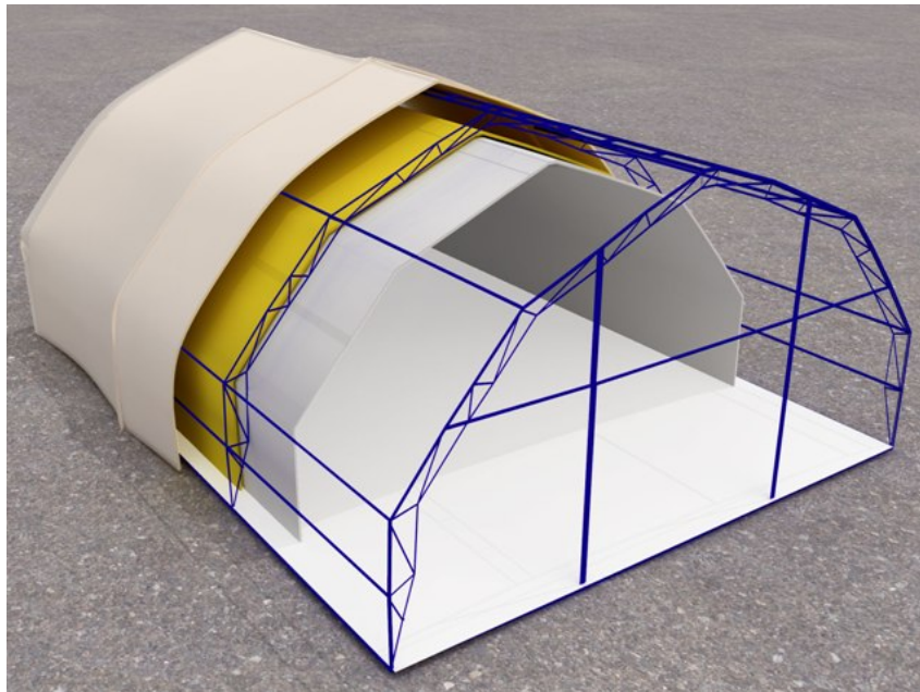
Fig. 5. Insulated two-membrane frame-tent structure [5]
