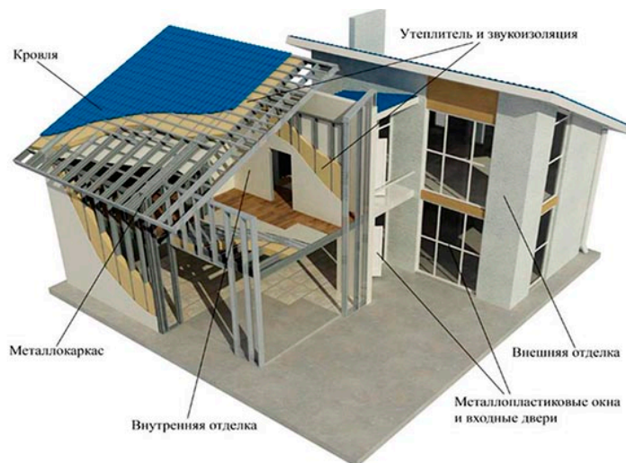
Fig. 1. Light-weight steel thin-walled structures [1]
