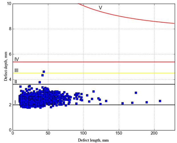
Figure 4. Express assessment of the level of danger of external defects of the «loss of metal» type
