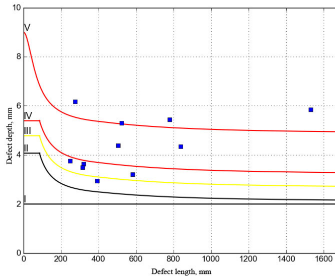
Figure 5. Express assessment of the level of danger of defects of the «pipe wall lamination» type
