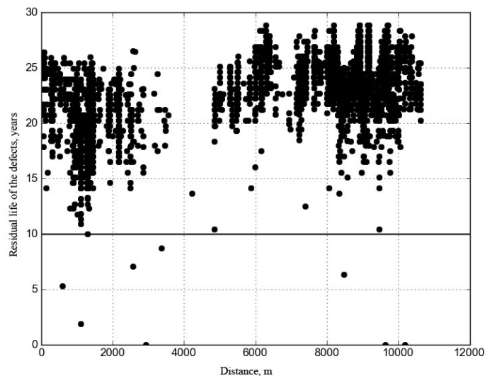
Figure 6. Residual life of the defective cross sections of the pipeline (assessments of true sizes of defects depths were used)
