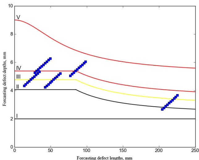
Figure 7. Forecasting express assessment of the level of danger of internal defects of the «loss of metal» type
