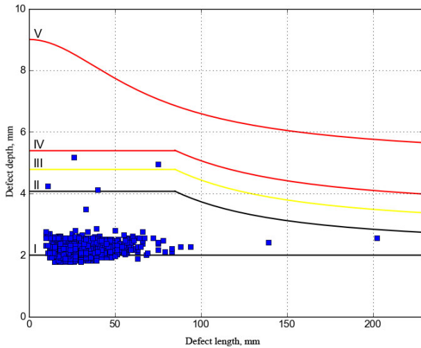
Figure 3. Express assessment of the level of danger of internal defects of the «loss of metal» type
