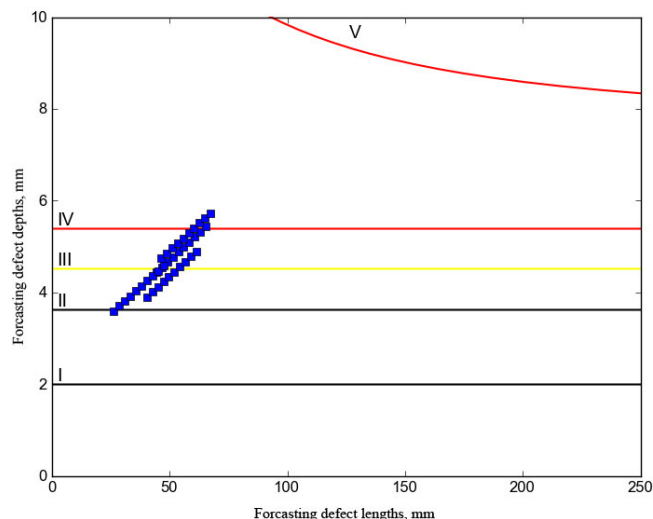
Figure 8. Forecasting express assessment of the level of danger of external defects of the «loss of metal» type
