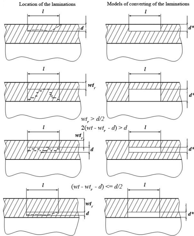
Figure 2. Location of the laminations and models of its converting to the surface «loss of metal» type defects
