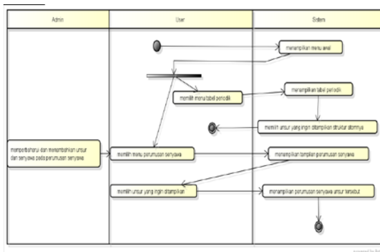
Gambar 2. Activity Diagram
