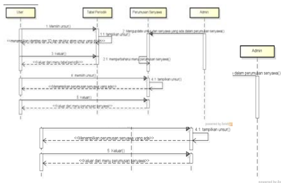
Gambar 3. Sequence Diagram
