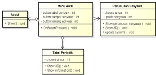
Gambar 4. Class Diagram
