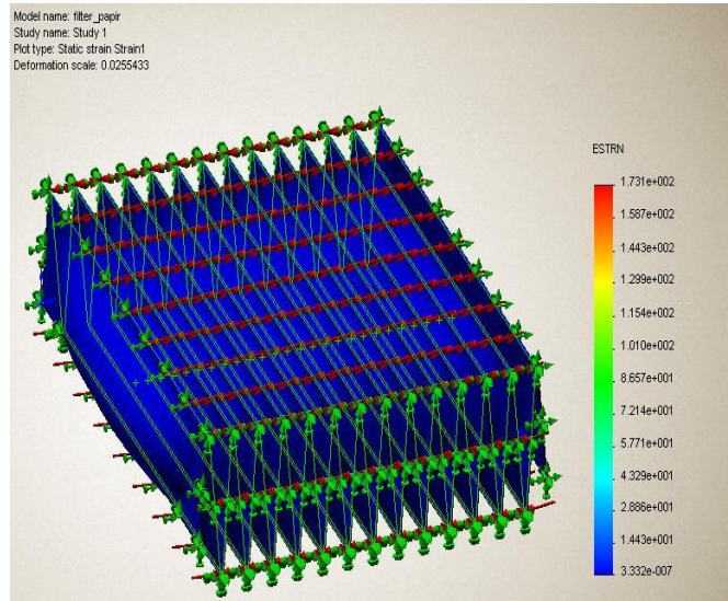
Fig. 6 Filter_paper-Study 1-Strain-Strain1
