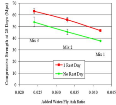
Fig.4.2. With Flyash adding.
