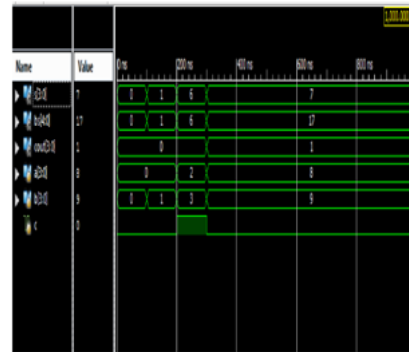
Fig.4.1. OUTPUT waveforms.
