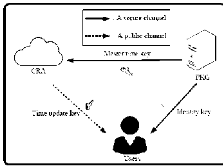
Fig.1. Proposed framework
