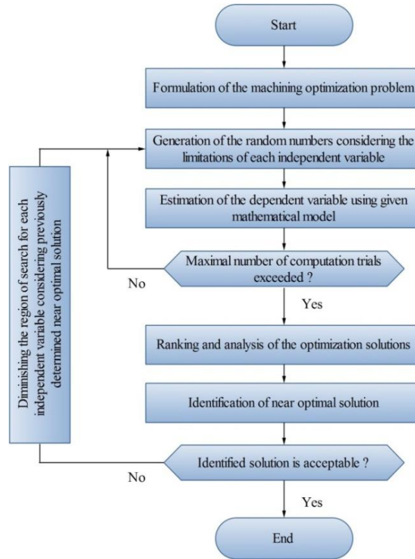
Fig. 1 Monte Carlo method flowchart for solving machining optimization problems
