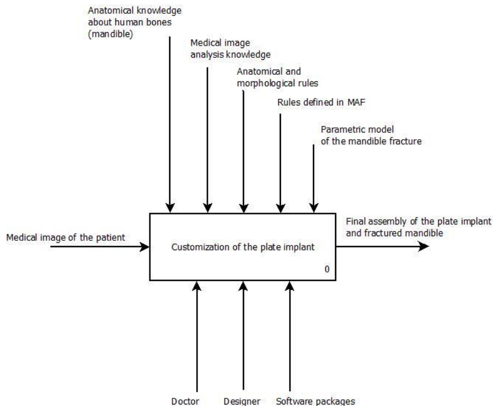
Fig. 1 Creation of the geometrical models of the plate implant and mandibular fracture – context diagram A-0
