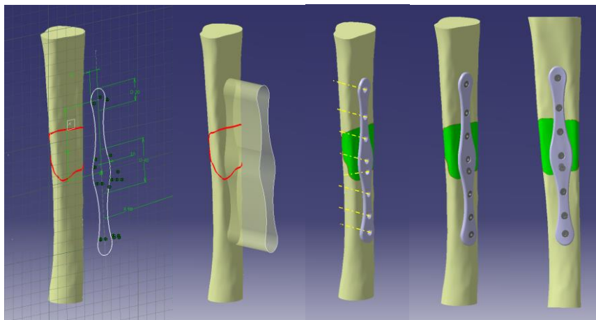
Fig. 15 Set bone-volumetric implant-fixation tile
