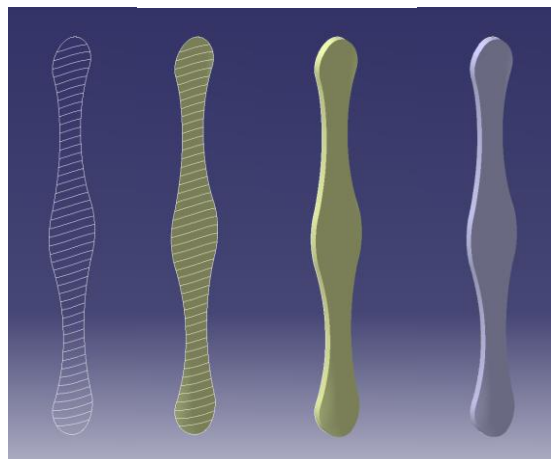
Fig. 11 Intersecting contour, 3D splines inside of the contour, extruded surface
