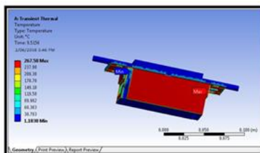
Fig.4.5. Temperature.
