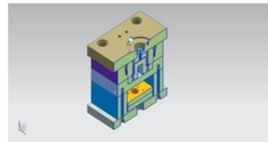
Fig.4.7. Assembly model.
