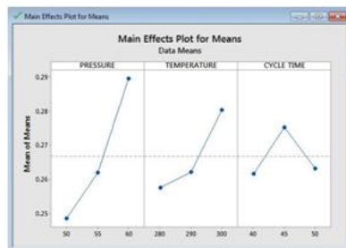
Fig.4.10. Effect of Injection Moulding machine parameters on force for Means.
