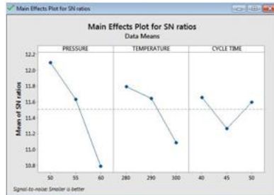
Fig.4.9. Effect of turning parameters on force for S/N ratio.
