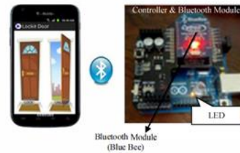
Fig. 4. Experimental set-up
