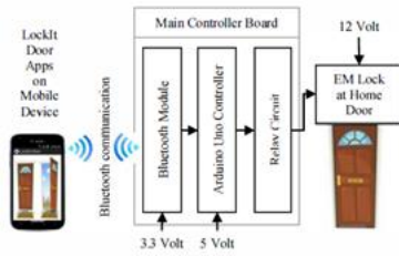
Fig. 1. System architecture
