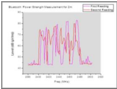
Fig: 5. Bluetooth power strength for 2m.
