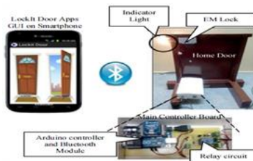
Fig. 3. Hardware set-up
