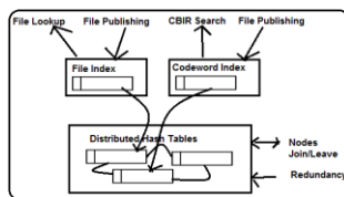
Fig.1. System Framework
