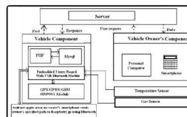
Fig.1.Proposed system framework
