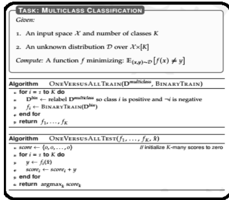
Fig.1.Algorithm
