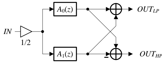
Fig. 2 IIR odd order filter realization as a parallel connection of two all-pass filters
