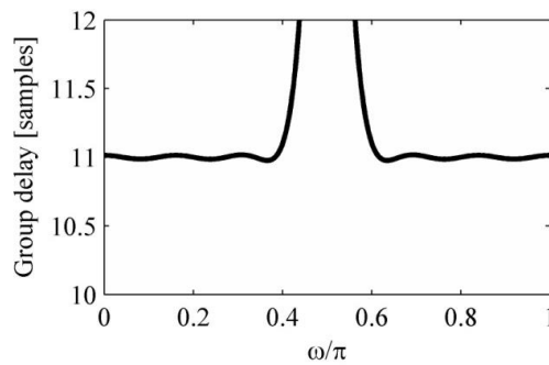
Fig. 4 Group delay of the filter designed by optimization algorithm [8]
