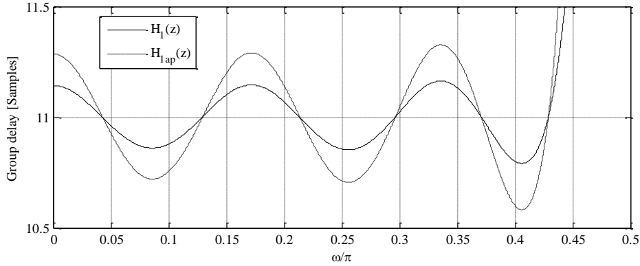
Fig. 14 The group delay of the all-pass branch H_{1ap}(z) and of the low-pass filter H_1(z) designed by the optimization method [8]
