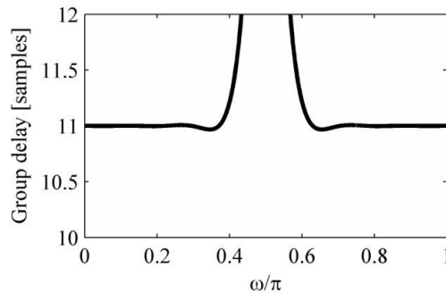
Fig. 6 Group delay of the filter designed by zero positioning algorithm [9, 10]
