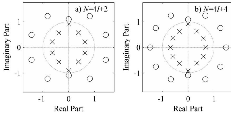
Fig. 7 Poles (x) and zeros (o) of the all-pass transfer function A_0(z) , a) filter order is N_0 = 4l + 2 , b) filter order is N_0 = 4l + 4
