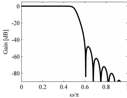
Fig. 5 Gain response of the filter designed by zero positioning algorithm [9, 10]
