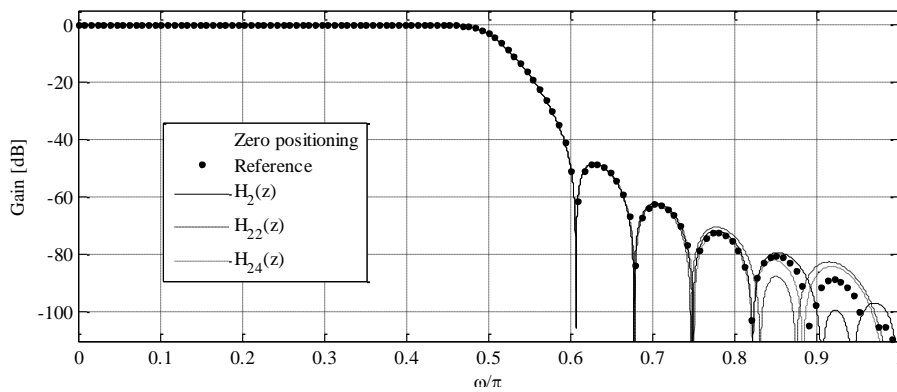
Fig. 12 The gains of the analyzed filters based on the low-pass stop-band zeros positioning [9, 10], for three different implementation of the all-pass branch A_0(z) , H_2(z) – direct implementation, H_{22}(z) – cascaded connection of the second order sections, H_{24}(z) – cascaded connection of the second and fourth order sections
