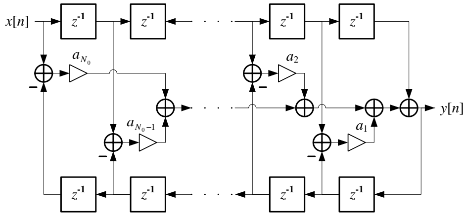
Fig. 8 All-pass filter structure with minimum number of multiplications ( N_0=4 )
