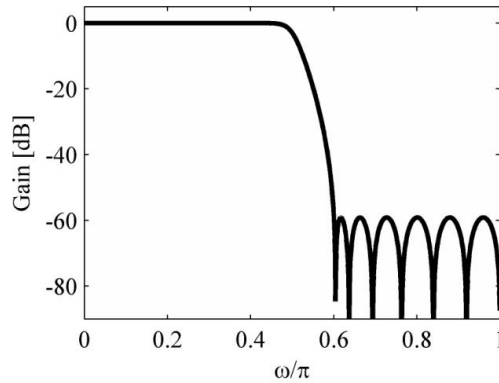
Fig. 3 Gain response of the filter designed by optimization algorithm [8]
