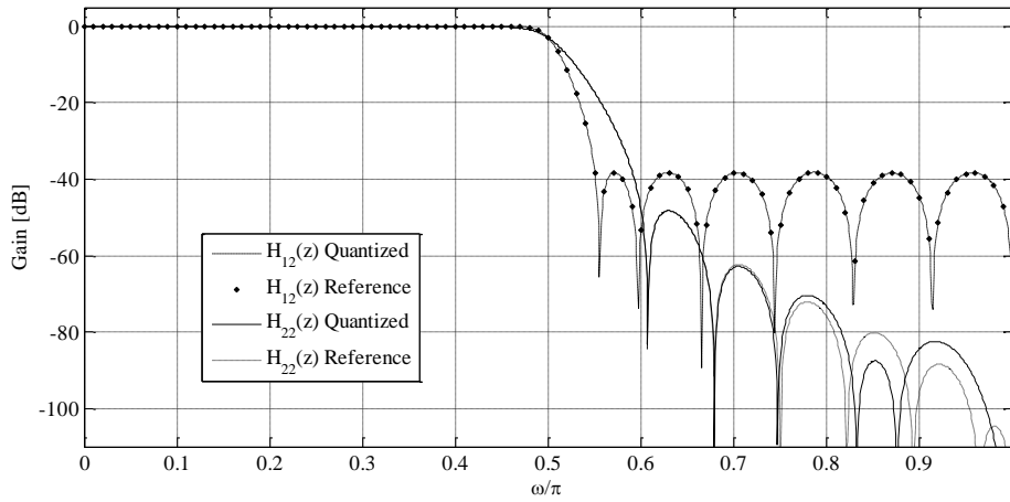
Fig. 11 The gains of the analyzed filters, H_{12}(z) – design method based on the optimization [8], H_{22}(z) – design method based on the low-pass stop-band zeros positioning [9, 10]
