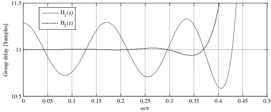
Fig. 13 The group delay of the analyzed filters, H_{12}(z) – design method based on the optimization [8], H_{22}(z) – design method based on the low-pass stop-band zeros positioning [9, 10]
