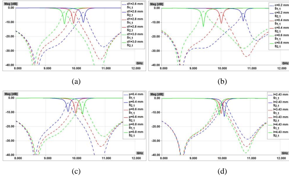
Fig. 2 Comparison of amplitude responses: (a) d_1 varies, (b) c varies, (c) p varies, (d) l varies
