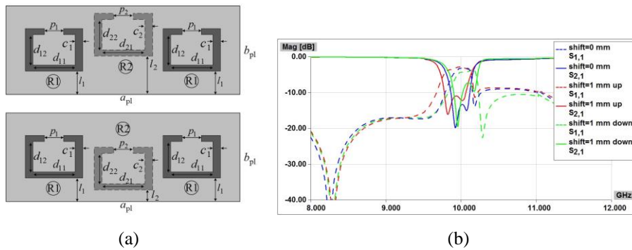
Fig. 7 Waveguide filter using E-plane insert with shifted central SRR: (a) models of the insert, (b) comparison of amplitude responses for various values of the shift
