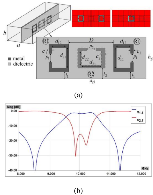
Fig. 9 Waveguide filter using E-plane insert with SRRs of various orientations: (a) 3D model and WIPL-D model of the insert, (b) amplitude response
