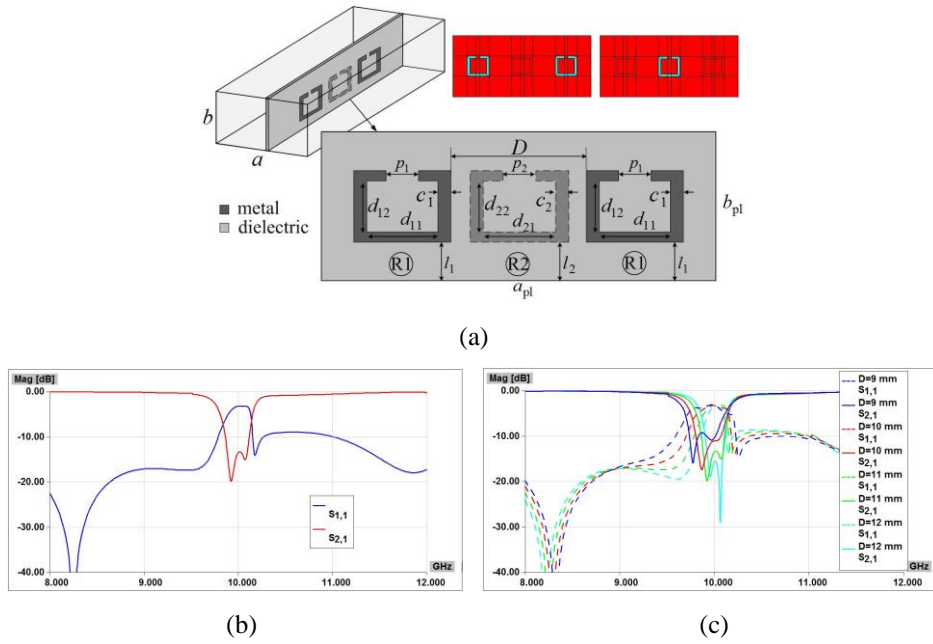
Fig. 6 Waveguide filter using E-plane insert with SRRs: (a) 3D model and WIPL-D model of the insert, (b) amplitude response, (c) comparison of amplitude responses for various values of distance D
