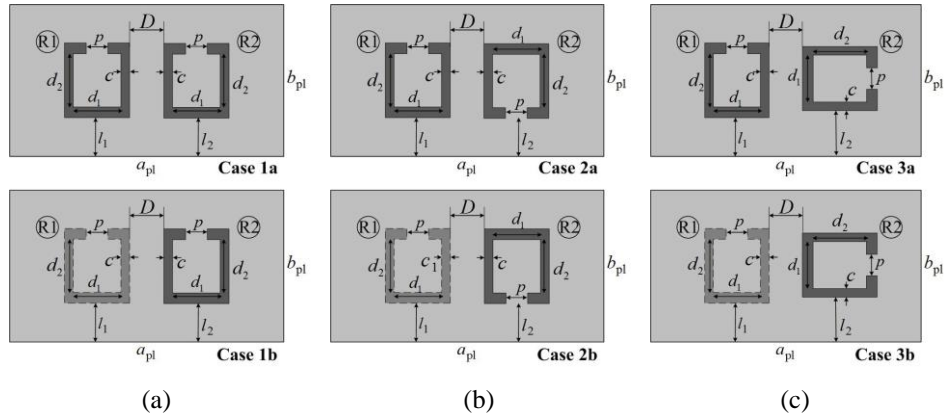
Fig. 4 SRR inserts used for coupling analysis: (a) case 1, (b) case 2, (c) case 3
