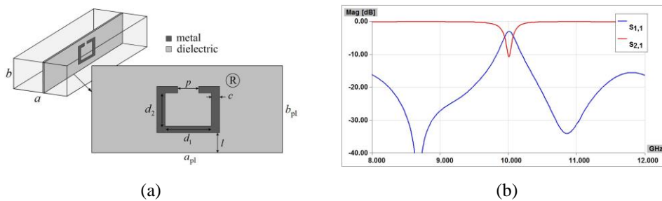
Fig. 1 Waveguide resonator using E-plane insert with a single SRR: (a) 3D model, (b) amplitude response
