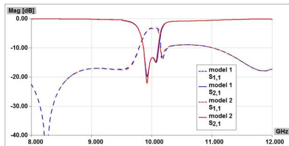
Fig. 8 Comparison of amplitude responses of E-plane bandstop filters with SRRs (model 1: double-sided printed-circuit insert, model 2: single-sided printed-circuit insert)
