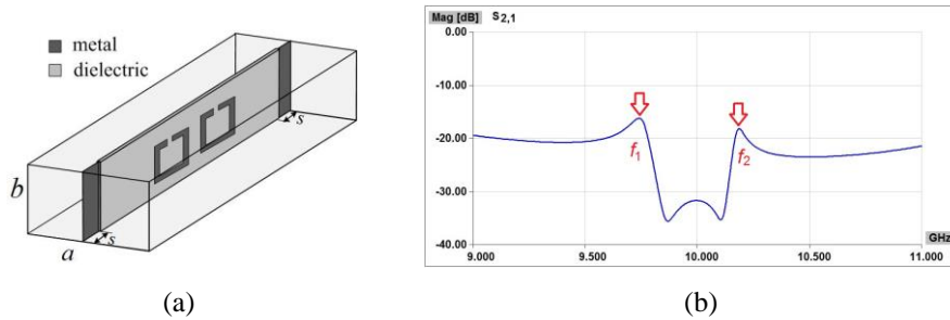
Fig. 3 Method of determining coupling coefficient: (a) 3D model with additional metal plates, (b) S_{21} characteristic with two local maxima
