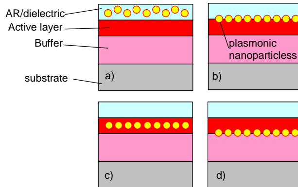
Fig. 4 Geometries for plasmonic scatterers for light trapping within photodetector. a) nanoparticles embedded in top dielectric; b) nanoparticles on top of the active region; nanoparticles embedded within the active region; d) nanoparticles on the back side
