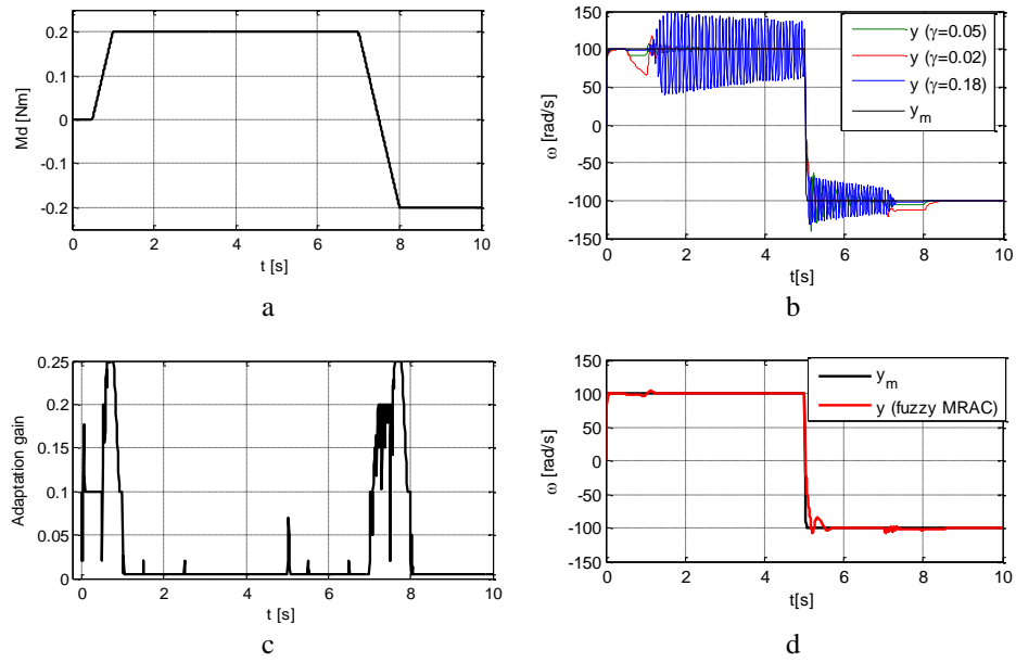
Fig. 4 Simulation results for tracking reference model:
