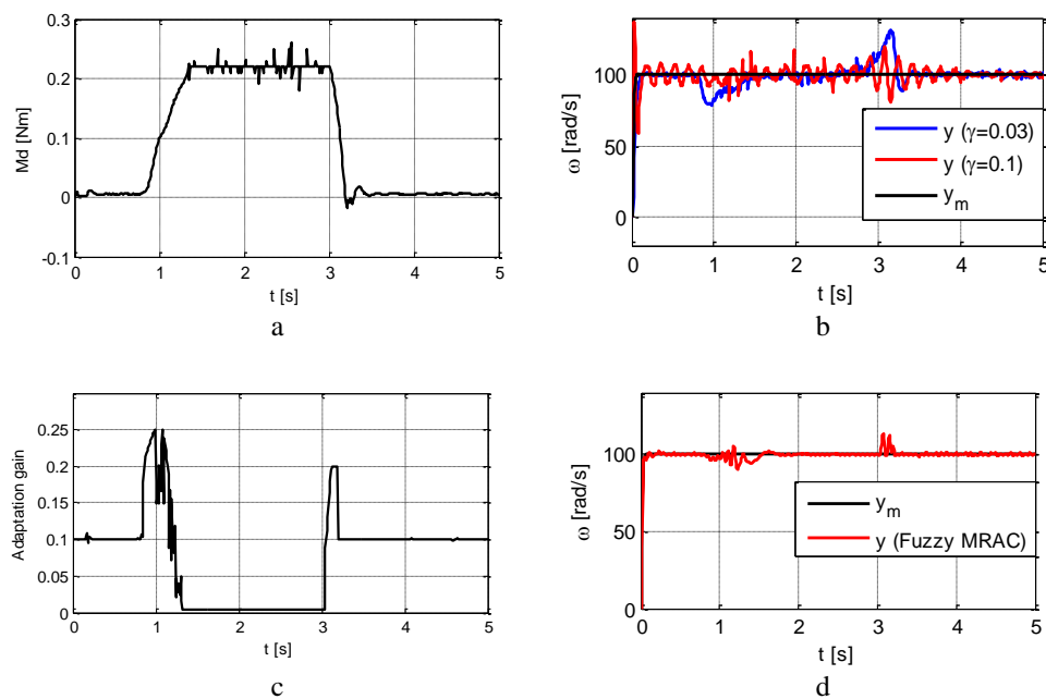
Fig. 8 Experimental results for tracking reference model:
