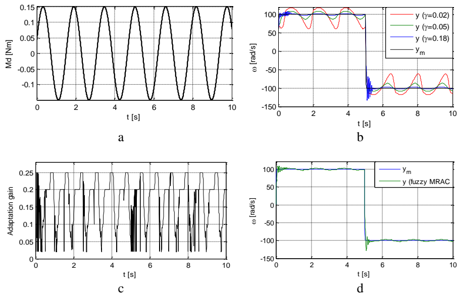
Fig. 5 Simulation results for tracking reference model:
