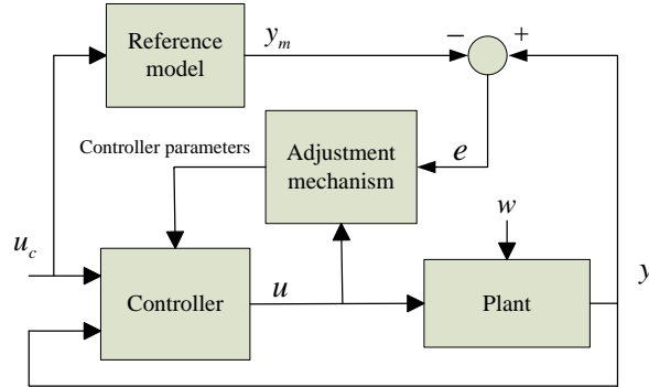
Fig. 1 Block diagram of model reference adaptive control
