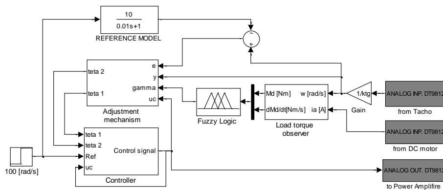
Fig. 7 Simulink model of fuzzy MRAC
