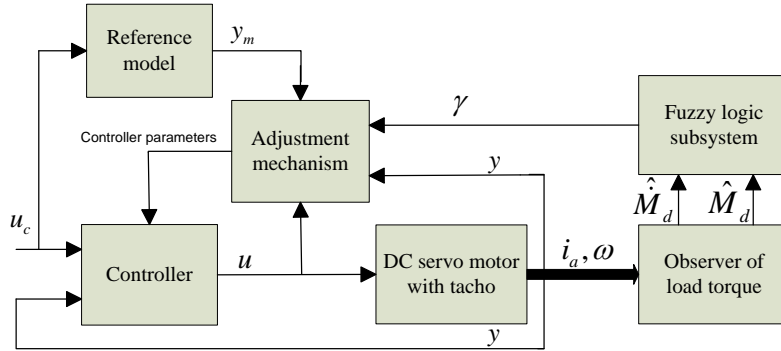
Fig. 2 Block diagram of fuzzy model reference adaptive control
