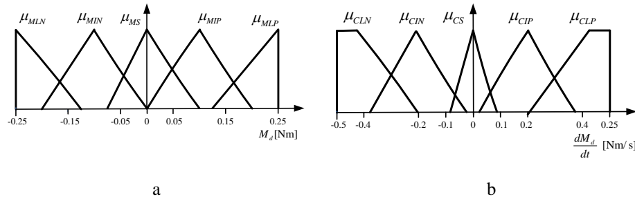
Fig. 3 Membership functions of: a) linguistic variable \hat{M} and b) linguistic variable \hat{CM}
