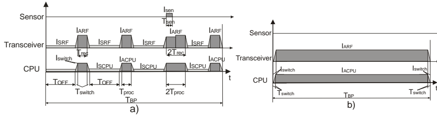
Fig. 7 Current profile of SN_3 's constituents during phases: a) Up_Sc ; b) Ne_Di_Re
