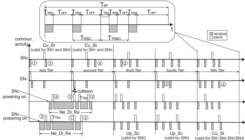
Fig. 3 Initialization phase with collision.
