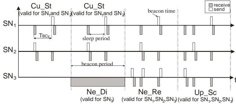
Fig. 1 DLDC-MAC rendezvous scheme
