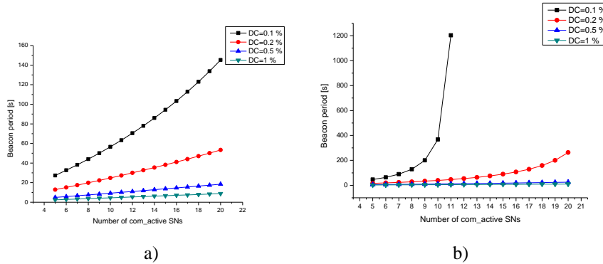
Fig. 6 Minimal duration of T_{BP} in terms of p , for DC factor as parameter: a) s_x = 10 ppm; b) s_x = 40 ppm
