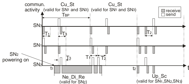
Fig. 2 Initialization phase without collisions.
