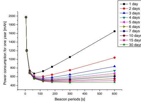
Fig. 9 Required battery capacity in terms of beacon period for different WSN scanning period
