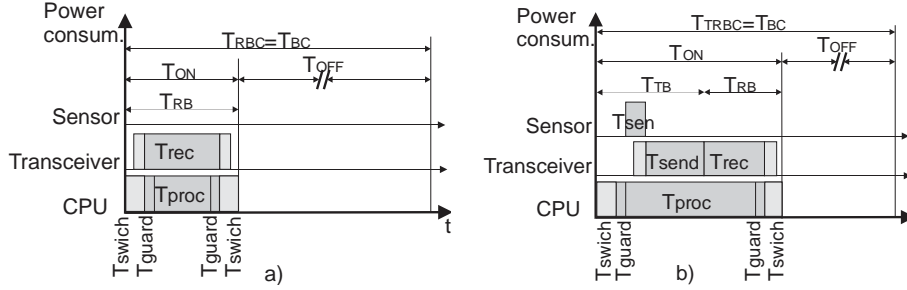
Fig. 4 Activity profile of SN during: a) receive beacon cycle; b) transmit-receive beacon cycle.
