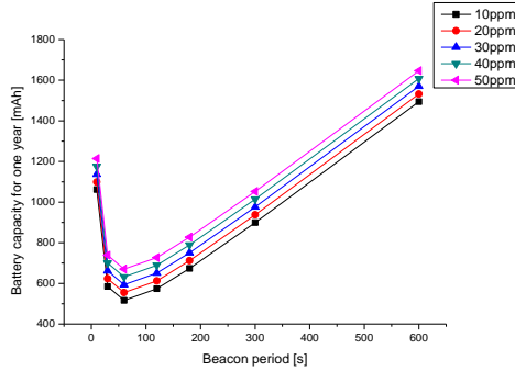
Fig. 8 Required battery capacity in terms of beacon periods with s_x as parameter
