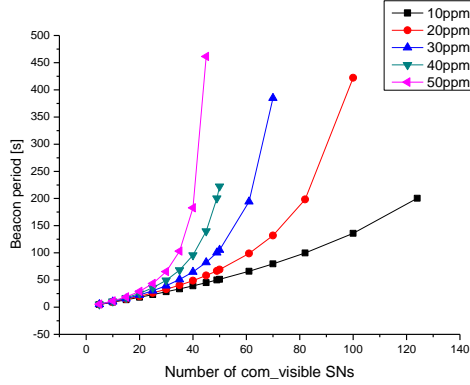
Fig. 5 Minimal duration of beacon period in terms of com_visible SNs for DC=0.5%
