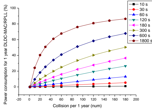
Fig. 10 Power comparison between DLDC-MAC and RPLL protocol for one year period in terms of number of collisions
