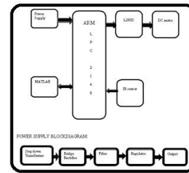
Fig.1. Block Diagram of Proposed System
