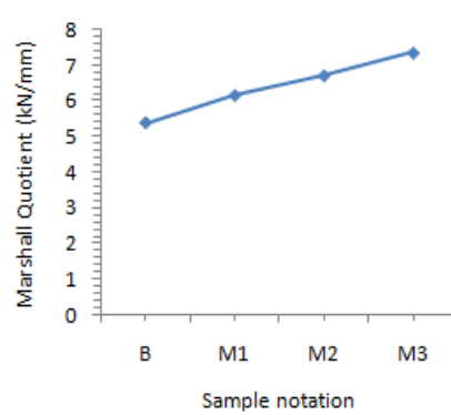
Fig. 11 Effect of MMT on Marshall Quotient
