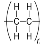
Fig. 1 Molecule of polyethylene
