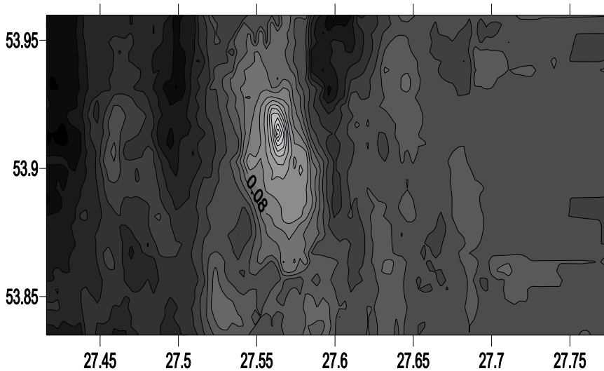
Figure 2. Block Kriging applied to Percentage Error.
