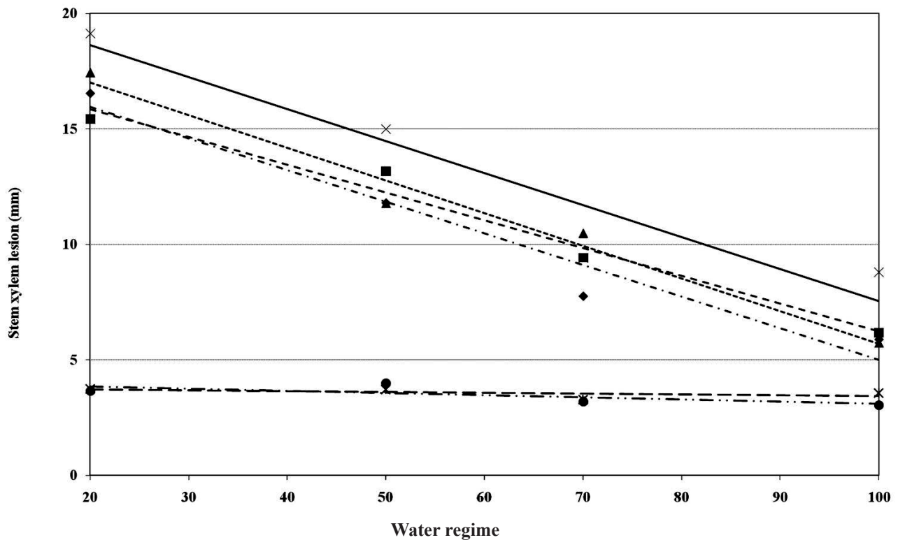
Figure 5. Linear regression lines [Eco-77 (— — —), water (· · · · ·), Lasiodiplodia theobromae (—), Neofusicoccum australe (— · — · —), N. parvum (— — —), Diplodia seriata (— — —)] fitted to the mean stem xylem lesions found in the stems of potted grapevines receiving the control treatments, Eco-77 (x) or water (•), or inoculated with N. australe (♦), D. seriata (■), N. parvum (▲), L. theobromae (x) and receiving 20, 50, 70% and optimal (100%) irrigation.
