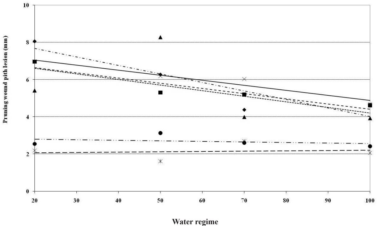
Figure 6. Linear regression lines [Eco-77 (— — —), water (— · · —), L. theobromae (—), N. australe (— · —), N. parvum (· · ·), D. seriata (— — —)] fitted to the mean pruning wound pith lesions observed in the stems of potted grapevines subjected to the control treatments, Eco-77 (x) or water (•), or inoculated with N. australe (♦), D. seriata (■), N. parvum (▲), L. theobromae (x) and receiving 20, 50, 70% and optimal (100%) irrigation.
