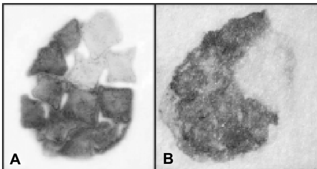
Fig. 3. Detection of Broad bean stain virus by TBIA in a group of 12 infected lentil seedlings, blotted together as one sample on nitrocellulose membrane (A) and on HP non-glossy plotter paper (B).
