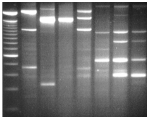
Fig. 2. Fragment lengths (bp) obtained after amplification with GT-primer. From left to right: 100 bp DNA Ladder, A730, 9133, 289612, 9421, T36, F1, AG-3.
