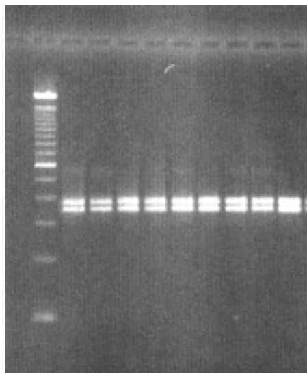
Fig. 1. Fragment lengths (bp) after endonuclease digestion with HinfI of the ITS regions including the 5.8S rDNA of Rhizoctonia solani isolates. From left to right: 100 bp DNA Ladder, R0297, R2297, R0397, R1397, R0497, R1497, R2497, R1697, TC1.
