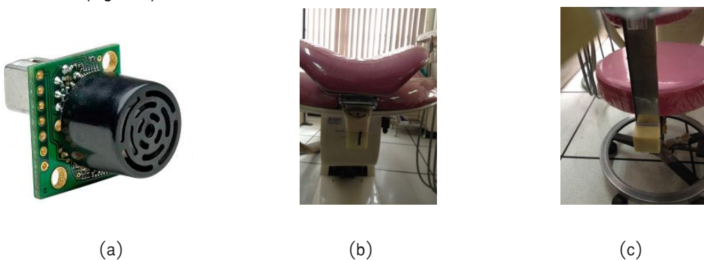
Figure 3. Ultrasonic sensors (a) ultrasonic sensor model MAXSONAR (b) head rest sensor container (c) dental chair sensor container
