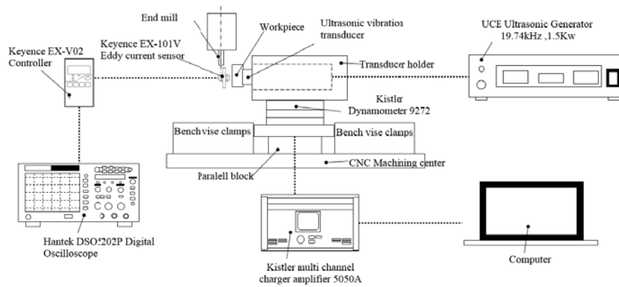
Figure 1 Schematic of experiment set up.
