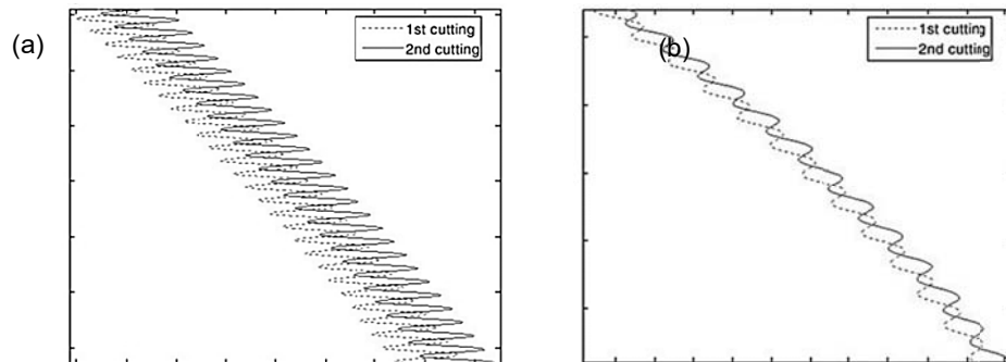
Figure 9 Trajectories of tool tips under different spindle speed (partial enlarged view). (a) Low cutting speed, (b) High cutting speed.
