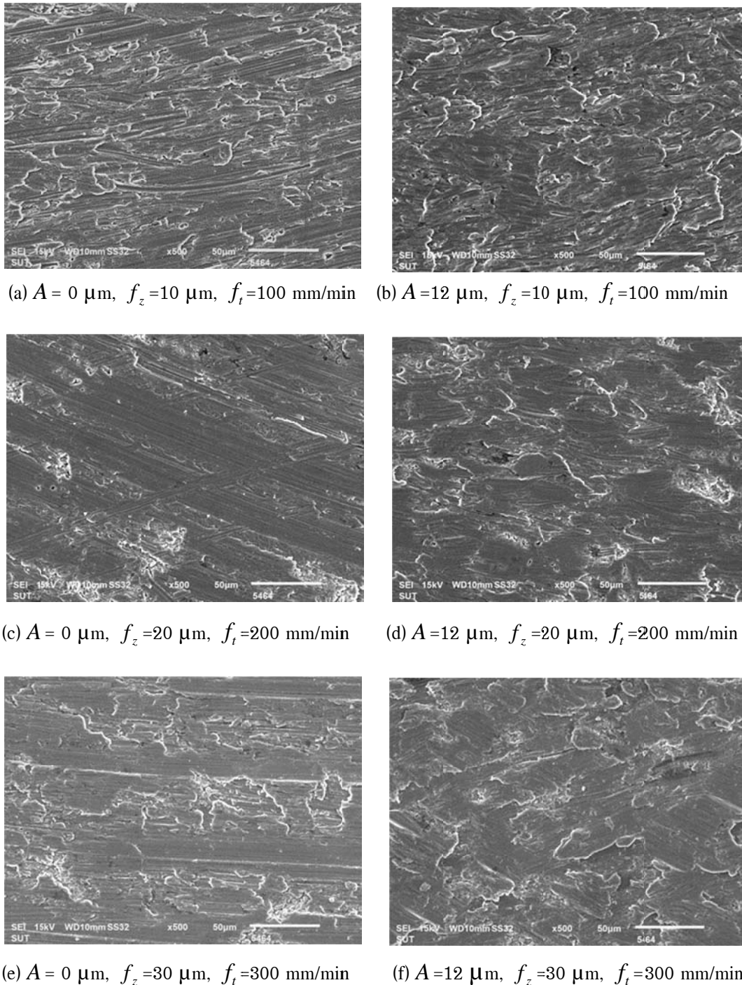
Figure 7 SEM photographs of finished surface at x500.
