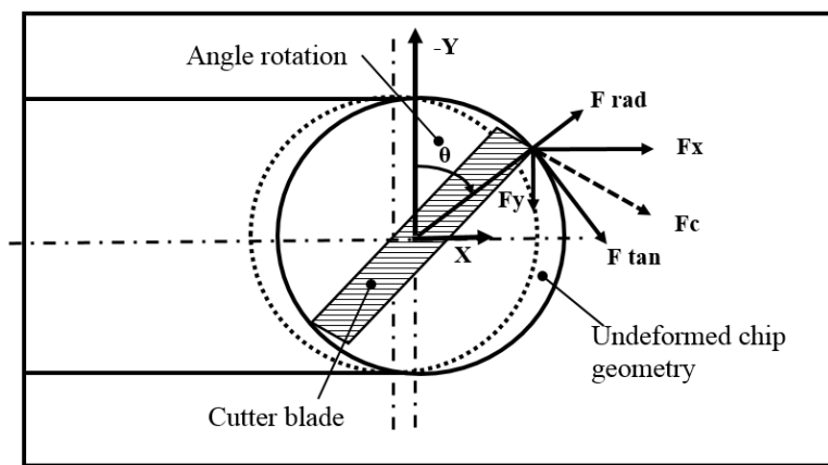
Figure 3 Cutting force components of slot milling.
