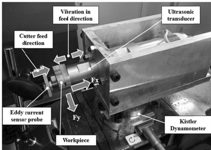
Figure 2 (a) Set up of workpiece and sensor for vibration amplitude measurement, (b) Output voltage from sensor measuring vibration amplitude ( 1 \mu\text{m}/7\text{mV} ) which shows the amplitude of 12 \mu\text{m}
