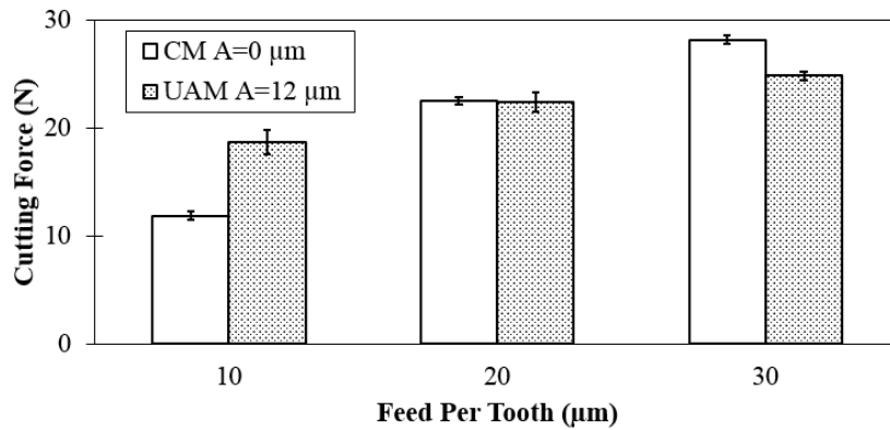
Figure 6 Average value of force in cutting direction ( F_c ) with different feeds per tooth.
