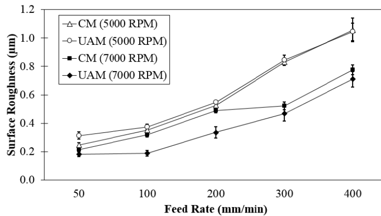
Figure 8 Average value of surface roughness with different cutting speed.
