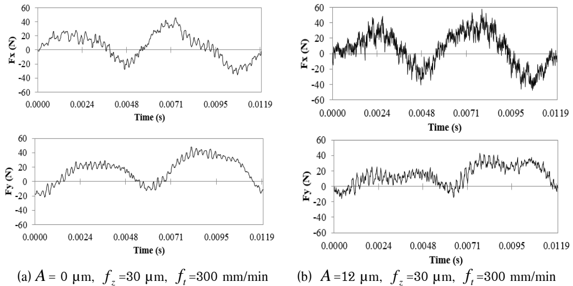
Figure 5 Experiment cutting force data in a cutting cycle.
