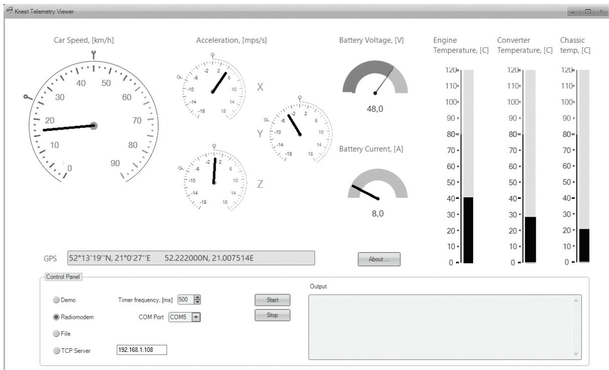
Fig. 7. Telemetric data visualization.
