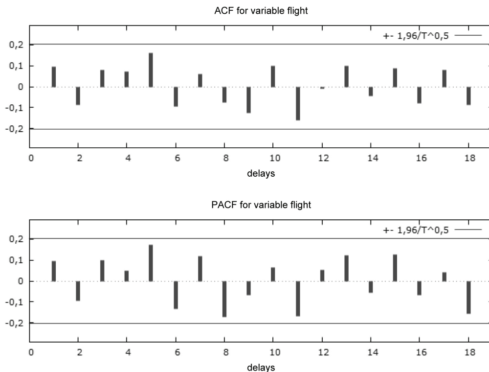
Fig. 2. Charts of ACF and PACF autocorrelation of researched series.
