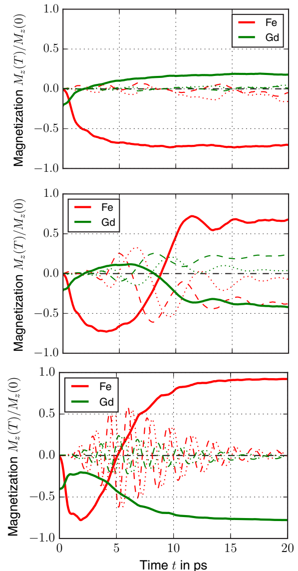
FIG. 2. The three possible time-relaxation scenarios for the sublattice magnetizations of a RE-TM layered system. The chosen values for T and Gd magnetization are indicated in Fig. 3. Top: Magnetization switches with respect to the initial configuration. Center: Both sublattice magnetizations change their signs twice, ending up back in the initial state. Bottom: No switching, i.e., the rare-earth layer magnetization does not change sign. Also shown are the transverse components (dotted and dashed lines). For the case of backswitching and no switching, these components are of the order of the magnitude of the magnetization.
