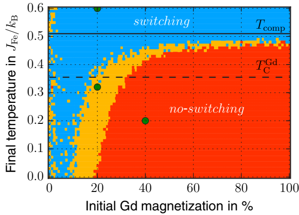
FIG. 3. Switching in a 3:2 layer sample after 40 ps. Color coding: Magnetization switches (cyan-blue), magnetization does not switch and returns to the initial state (red), and both magnetizations change their sign twice, ending up in the initial state (backswitching) (yellow-orange). The compensation temperature T_{\text{comp}} is indicated by a solid black line; the Curie temperature T_C^{\text{Gd}} of the isolated Gd layer is indicated by a dashed black line. The three points indicate the chosen values for the scenarios in Fig. 2.
