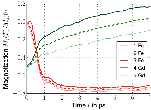
FIG. 5. Layer-resolved magnetization dynamics for switching in a 3:2 layer sample. The Gd layer is demagnetized to 50% of its zero-temperature value. The bold lines correspond to the layers at the Gd-Fe interface and the dashed lines show the average value for Gd or Fe. The temperature is T = 0.5 J_{\text{Fe}}/k_{\text{B}} .
