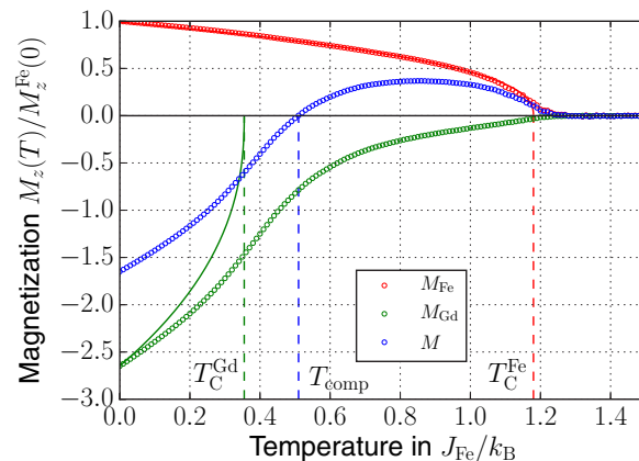
FIG. 1. Temperature-dependent equilibrium magnetization for a bilayer with three monolayers of Fe and two monolayers of Gd. The magnetization of the element with the stronger intralayer exchange interaction, in this case Fe, closely follows the shape of a ferromagnet with its Curie temperature T_C^{\text{Fe}} close to the Curie temperature of the coupled system. The element with the weaker intralayer exchange interaction, in this case Gd, exhibits magnetic ordering above its own bulk Curie temperature, T_C^{\text{Gd}} , due to the interaction with the other sublattice. The chosen ratio of layer thicknesses leads to a larger magnetic moment of the Gd layer at low temperatures and, consequently, to a magnetic compensation point at a temperature T_{\text{comp}} which is slightly above the bulk Curie temperature of the Gd.
