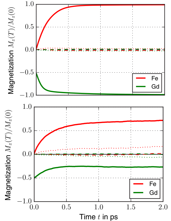
FIG. 4. Strong dissipation ( \alpha = 1 ) in a 3:2 layer sample, implying no conservation of angular momentum. The relaxation does not lead to a TFMLS either at low temperature where the Gd magnetization increases or at high temperature where it decreases. Top: T < T_C^{\text{Gd}} . Bottom: T_C^{\text{Gd}} < T < T_C^{\text{Fe}} . Also shown are the transverse components (dotted and dashed lines) which remain small for both cases.
