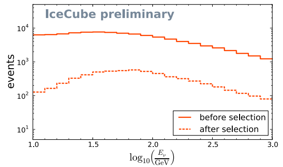
Figure 3: Energy spectrum of the simulated \nu_\mu after the online filter (solid) and in the final event sample (dashed), assuming standard oscillation parameters \Delta m^2_{32} = 2.4 \cdot 10^{-3} \text{eV}^2 and \sin^2(2\theta_{23}) = 1.0 .
