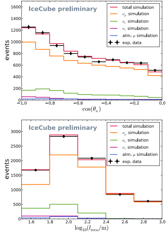
Figure 9: Distributions of reconstructed zenith angle and track length, with best-fit oscillation and nuisance parameters.
