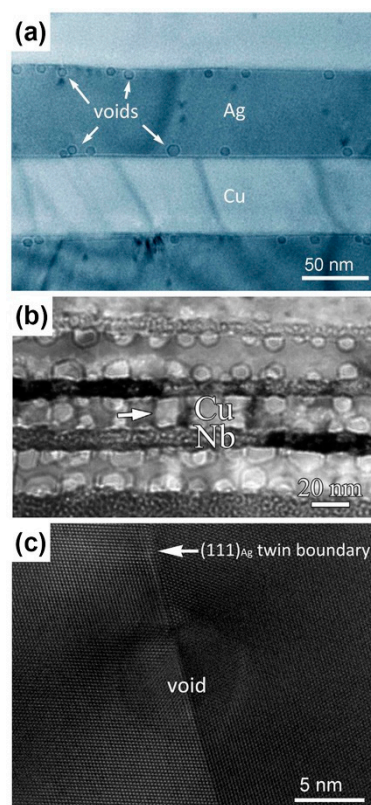
Figure 6. (a) Over-focus TEM image of the Cu/Ag composite after He ion irradiation at 450 °C [33]. (b) Under-focus TEM image of the ARB Cu/Nb nanolayered composites after He ion irradiation at 450 °C [22]. (c) High resolution transmission electron microscopy (HRTEM) image shows void wetting of a coherent (111) Ag twin boundary [33].
