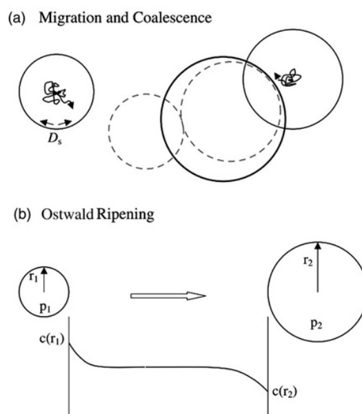
Figure 3. Schematic illustration of the two main bubble coarsening mechanisms, (a) migration and coalescence via surface diffusion, (b) Ostwald ripening due to He fluxes driven by differences in the thermal equilibrium He concentrations in the vicinity of small and large bubbles [8].
