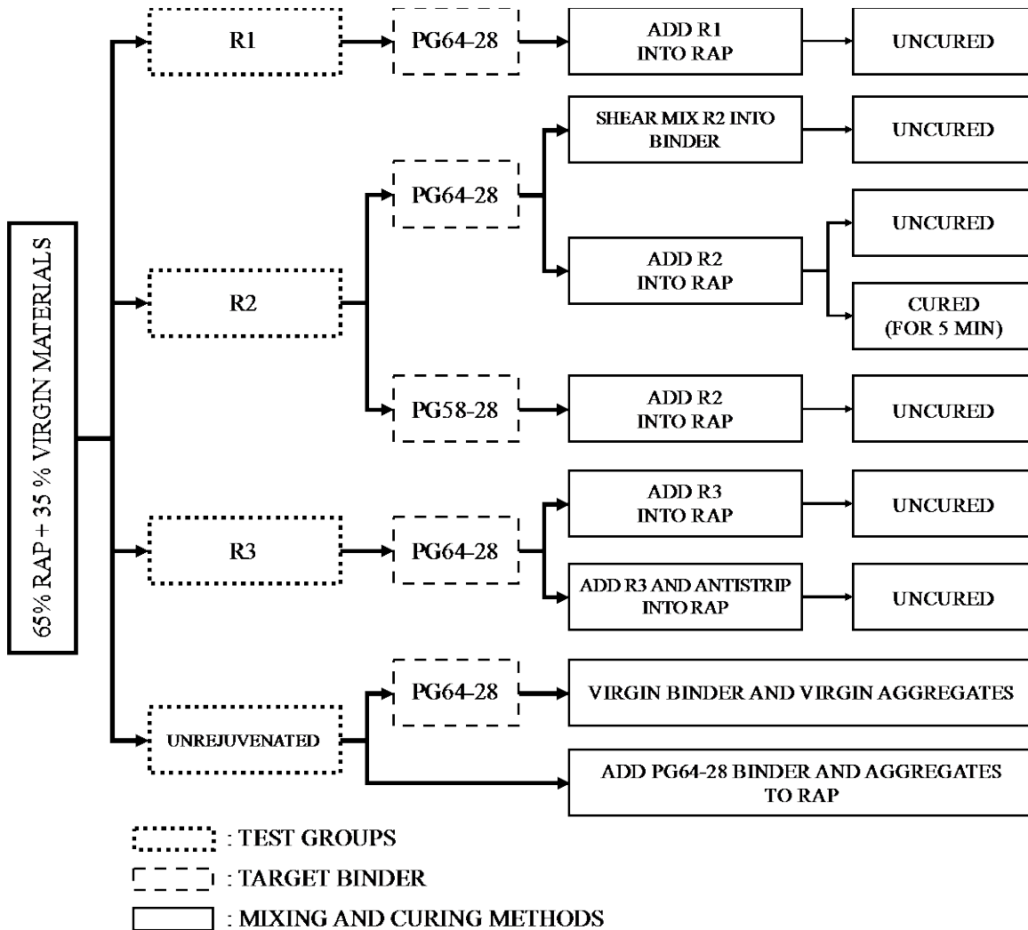
Figure 1-2. Testing plan designed asphalt mixture.
