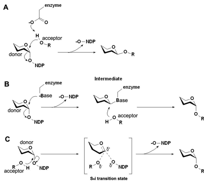
Figure 1. Schematic diagram showing possible mechanisms for glycosyltransferases that utilize a nucleotide-diphospho-sugar as a donor substrate [Adapted from (Davies, 2001)] Inverting glycosyltransferases probably follow a direct displacement mechanism in which a general base assists in the deprotonation of the reactive hydroxyl of the sugar acceptor and then acts as the nucleophile to attack the sugar donor (Figure 1A). In retaining glycosyltransferases, the reaction involves a double displacement with the formation of a covalent intermediate (Figure 1B). Another mechanism proposed for retaining glycosyltransferases suggests that the enzyme utilizes an S_Ni transition state in which the approach of the attacking acceptor and the leaving donor are on the same side of the sugar ring (Figure 1C)
