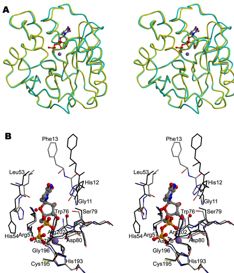
Figure 3. The structure of A64R complexed with UDP
