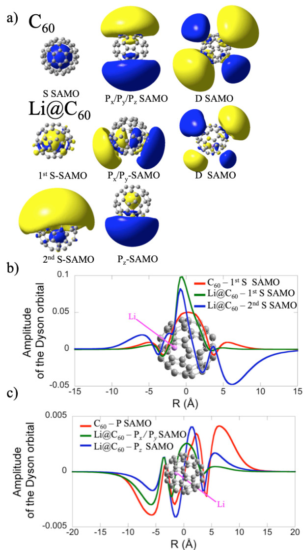
Fig. 2: a) Dyson orbitals of the S-, P- and D-SAMO electronic states of C_{60} and of the most stable isomer of Li@C_{60} computed at the TDDFT/CAM-B3LYP level (see computational details for the basis set). b) Amplitude of the S-SAMO Dyson orbitals along the molecular axis z that passes through the centre of the cage and the Li atom. The amplitude of the 2 nd S-SAMO has been multiplied by a factor -50 c) Amplitude of the P_x , P_y and P_z -SAMO Dyson orbitals along the z axis (taken at x=y=0 ) for the P_z component and along the x axis for the P_x component of the P-SAMO.
