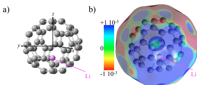
Fig. 1: a) Equilibrium geometry of the lowest energy isomer of Li@C_{60} computed at the DFT level with the B3LYP functional (see computational details). b) Electrostatic potential surface mapped on the electronic density surface for an isovalue of 0.001 |e|/\text{Å}^3 .
