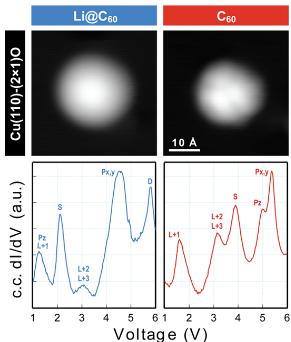
Fig. 9(a) Image of isolated fullerene molecules deposited on Cu(110)-(2×1)-O obtained for a bias voltage of +2.5 V and the corresponding constant-current dI/dV spectra. Left: Li@C 60 ; Right: C 60 . The assignment marked on the C 60 spectrum is identical to that of Reecht et al. 46
