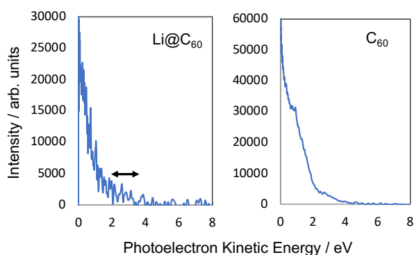
Fig. 6. Photoelectron spectra obtained at 267 nm. Left: Li@C_{60} . Right: C_{60} . No clear structure associated with SAMO states can be seen in the C_{60} spectrum with only a slight, very low intensity indication in the Li@C_{60} spectrum. No thermal/unresolved background has been subtracted for this data.
