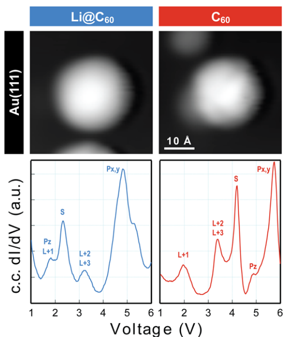
Fig. 10. Image of two isolated fullerene molecules deposited on Au(111) obtained for a bias voltage of +2.5 V and the corresponding constant-current dI/dV spectra. Left: \text{Li}@C_{60} ; Right: C_{60} . The assignment marked on the C_{60} spectrum is identical to that of Reecht et al. 46
