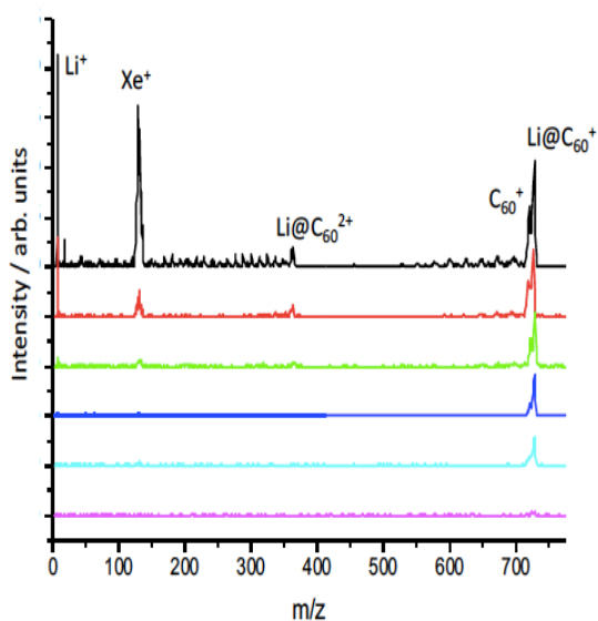
Fig. 3. Mass spectra obtained from ionising the effusive molecular beam at 620 K with 540 nm, 35 \pm 10 fs, as a function of laser intensity (increasing from bottom, 4.4 \text{ TWcm}^{-2} , to top, 29 \text{ TWcm}^{-2} ). The Xe + peak is present for calibration purposes. The photoelectron spectra discussed in section 3.2 were obtained for conditions corresponding to the 3 rd spectrum from the bottom ( 10 \text{ TWcm}^{-2} ).
