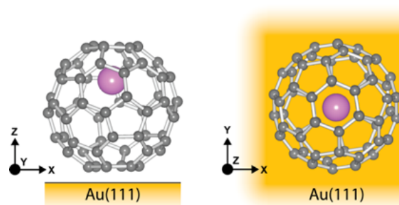
Fig. 11. Illustration of \text{Li@C}_{60} on \text{Au}(111) showing the most energetically favourable orientation. (a) side view (b) top view.
