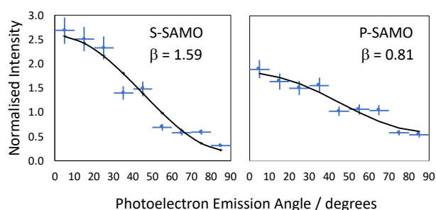
Fig. 7. Representative data illustrating the determination of the anisotropy parameter \beta from the angular dependence of SAMO peak intensities. The data was obtained at a wavelength of 540 nm for peaks with a photoelectron kinetic energy of 0.29 \pm 0.02 eV ( E_{\text{Bind}} = 2.00 \pm 0.02 eV, S-SAMO) and 0.87 \pm 0.06 eV ( E_{\text{Bind}} = 1.43 \pm 0.06 eV, P-SAMO).
