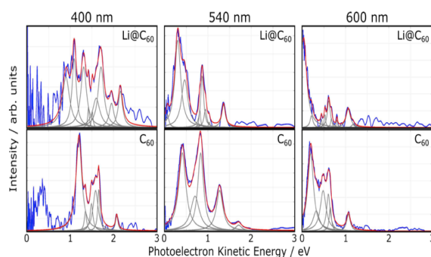
Fig. 5. Angle-integrated photoelectron spectra obtained for Li@C_{60} shown for three representative wavelengths (blue lines). The corresponding C_{60} spectra (used to subtract the C_{60} component from the raw Li@C_{60} spectra) are shown for comparison. The grey dashed lines indicate the Lorentzian fit functions and the red lines show the sum of these functions. In all cases the thermal background signal was removed.
